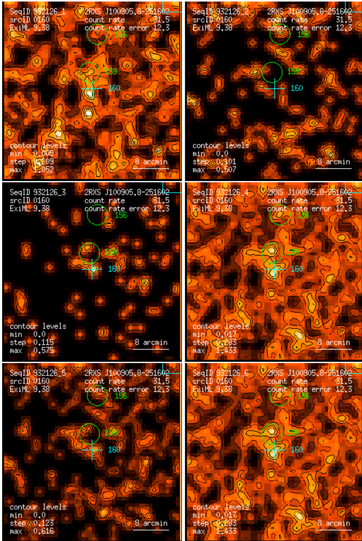
Figure 160: RASS 932126: detection 0160: band rate images, Gaussian filter: (1) PSPC channels 11 – 41, (2) 52 – 90, (3) 91 – 201, (4) 11 – 235, (5) 52 – 201, (6) 11 – 201. Broad band rates in counts/ks. Band rate contour levels in counts/ks/arcmin 2 .
