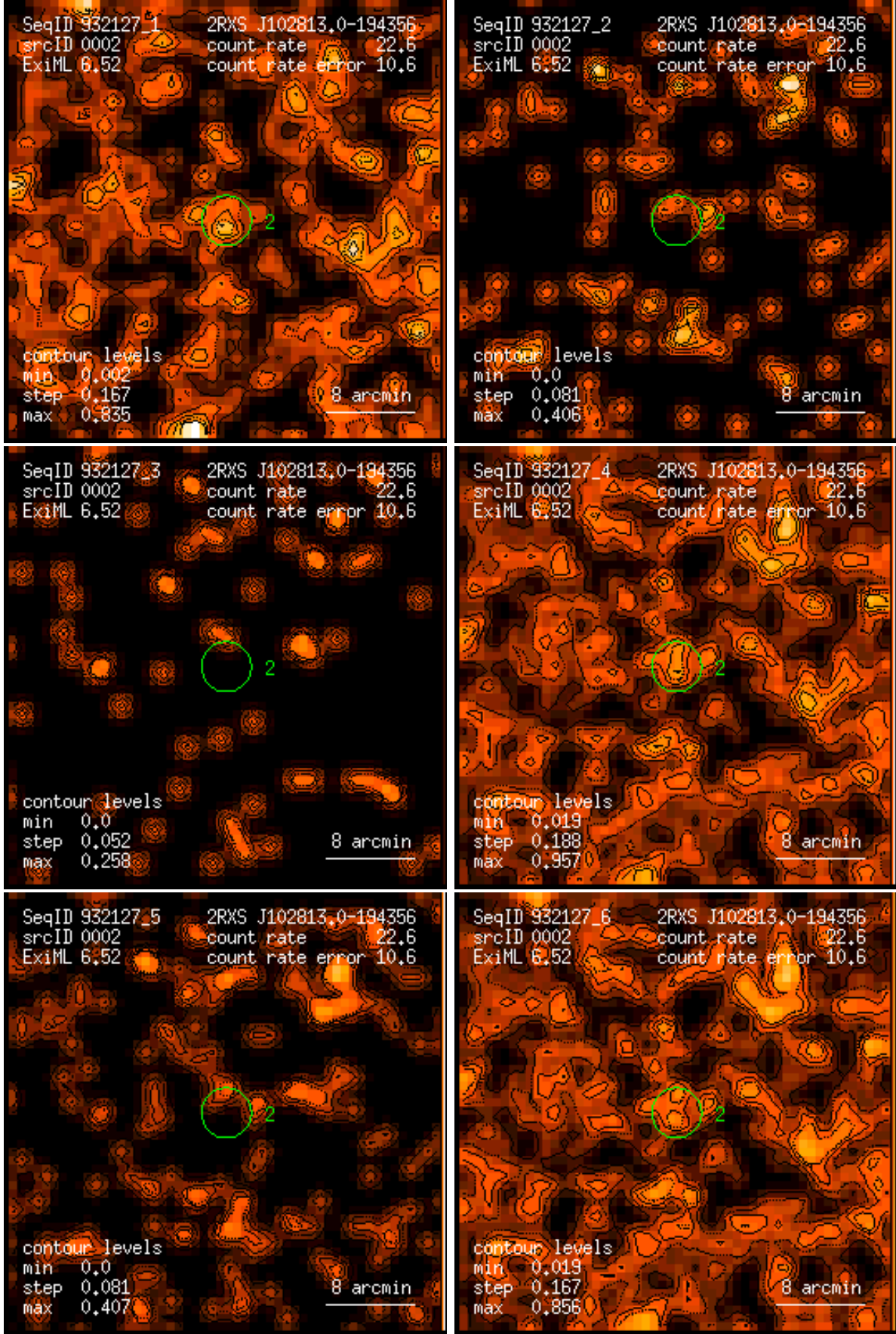
Figure 2: RASS 932127: detection 0002: band rate images, Gaussian filter: (1) PSPC channels 11 – 41, (2) 52 – 90, (3) 91 – 201, (4) 11 – 235, (5) 52 – 201, (6) 11 – 201. Broad band rates in counts/ks. Band rate contour levels in counts/ks/arcmin 2 .
