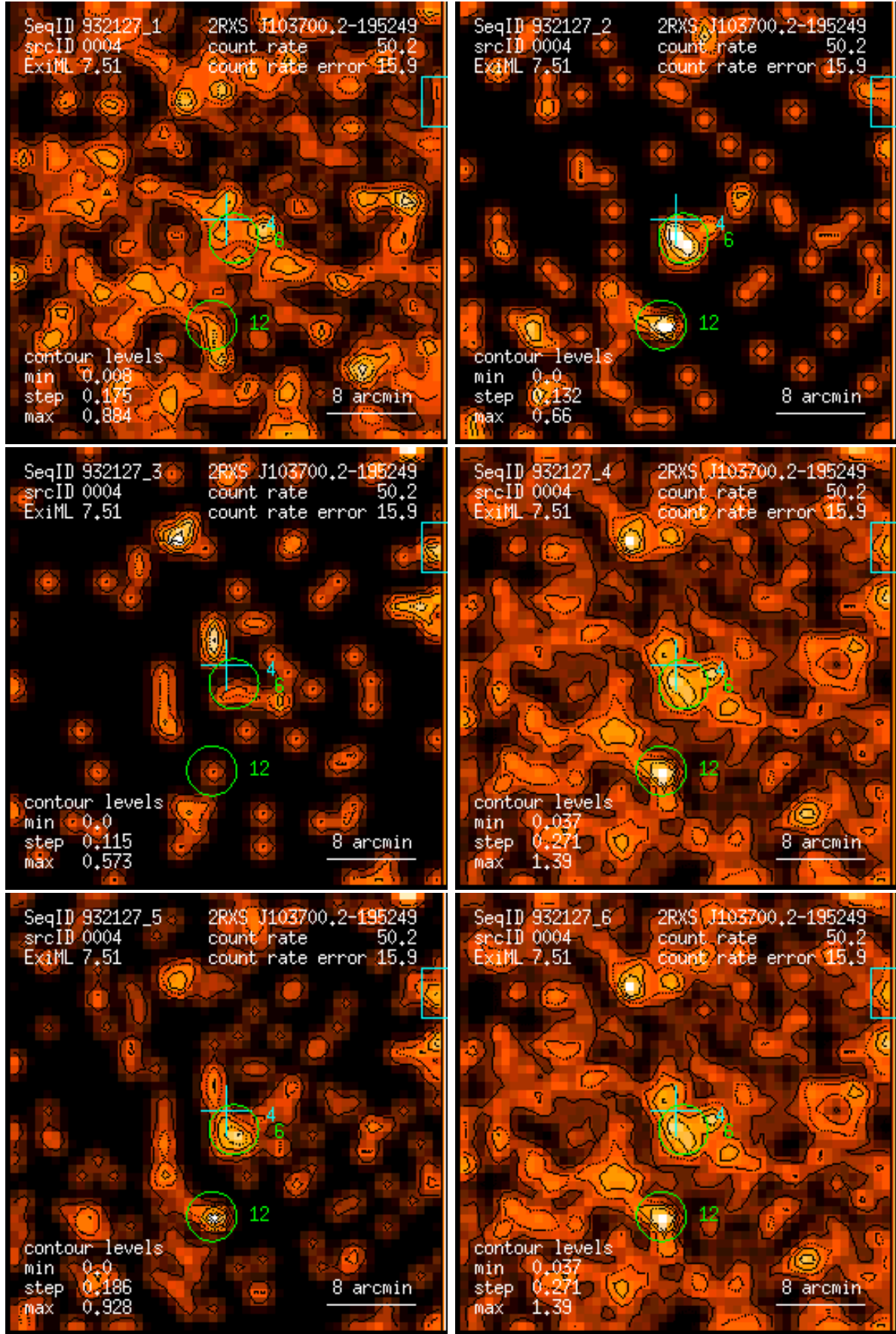
Figure 4: RASS 932127: detection 0004: band rate images, Gaussian filter: (1) PSPC channels 11 – 41, (2) 52 – 90, (3) 91 – 201, (4) 11 – 235, (5) 52 – 201, (6) 11 – 201. Broad band rates in counts/ks. Band rate contour levels in counts/ks/arcmin 2 .
