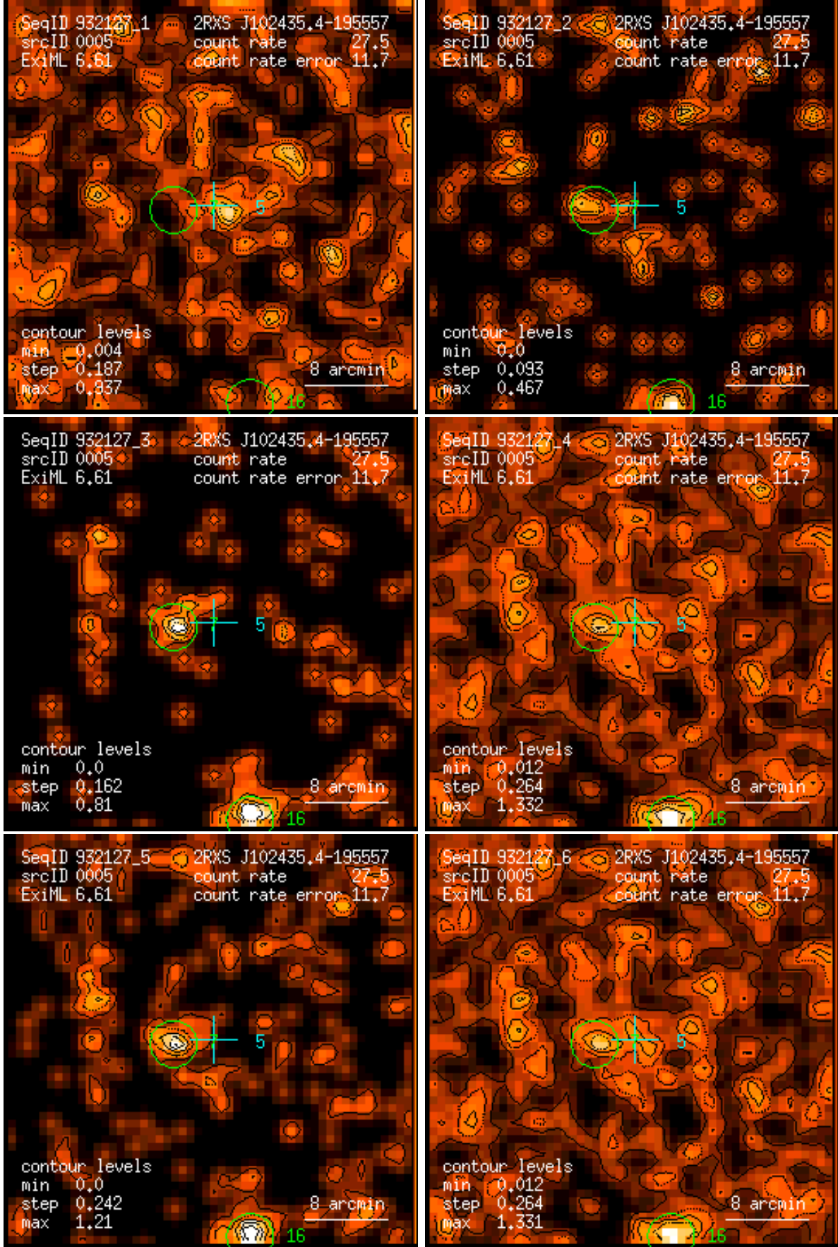
Figure 5: RASS 932127: detection 0005: band rate images, Gaussian filter: (1) PSPC channels 11 – 41, (2) 52 – 90, (3) 91 – 201, (4) 11 – 235, (5) 52 – 201, (6) 11 – 201. Broad band rates in counts/ks. Band rate contour levels in counts/ks/arcmin 2 .
