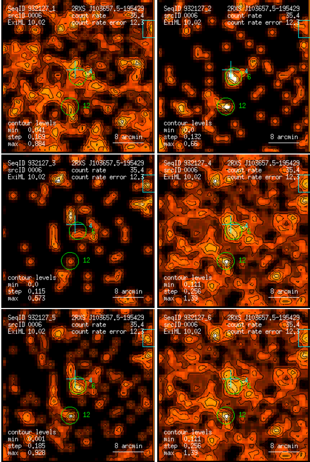
Figure 6: RASS 932127: detection 0006: band rate images, Gaussian filter: (1) PSPC channels 11 – 41, (2) 52 – 90, (3) 91 – 201, (4) 11 – 235, (5) 52 – 201, (6) 11 – 201. Broad band rates in counts/ks. Band rate contour levels in counts/ks/arcmin 2 .
