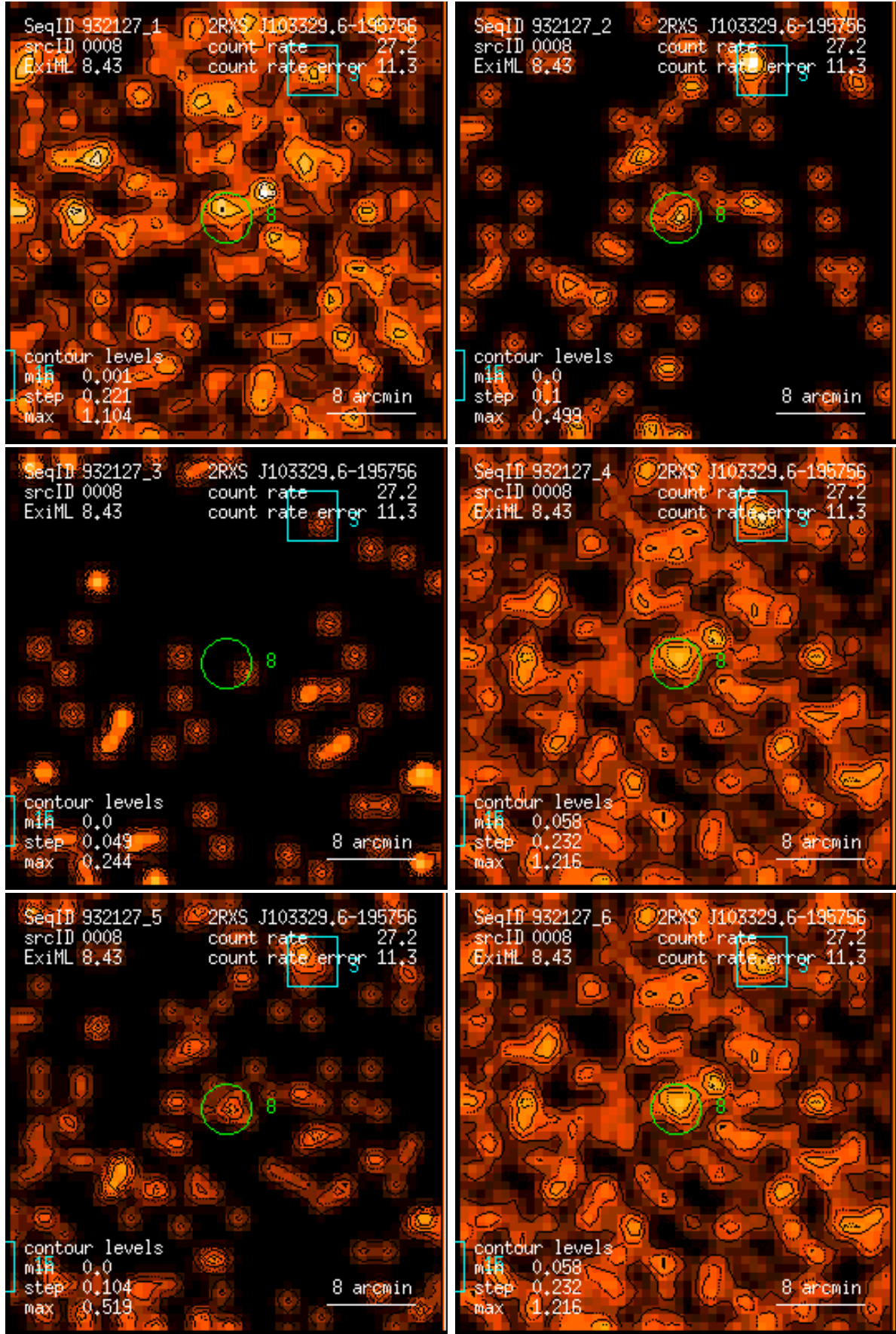
Figure 8: RASS 932127: detection 0008: band rate images, Gaussian filter: (1) PSPC channels 11 – 41, (2) 52 – 90, (3) 91 – 201, (4) 11 – 235, (5) 52 – 201, (6) 11 – 201. Broad band rates in counts/ks. Band rate contour levels in counts/ks/arcmin 2 .
