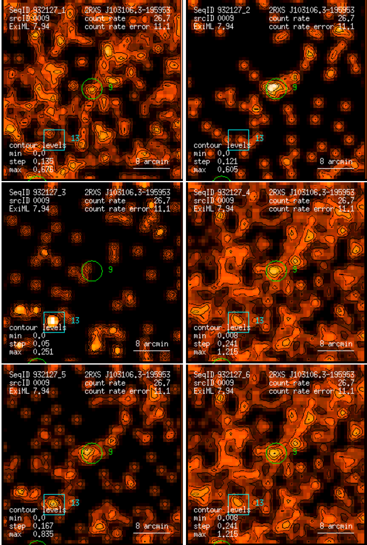
Figure 9: RASS 932127: detection 0009: band rate images, Gaussian filter: (1) PSPC channels 11 – 41, (2) 52 – 90, (3) 91 – 201, (4) 11 – 235, (5) 52 – 201, (6) 11 – 201. Broad band rates in counts/ks. Band rate contour levels in counts/ks/arcmin 2 .
