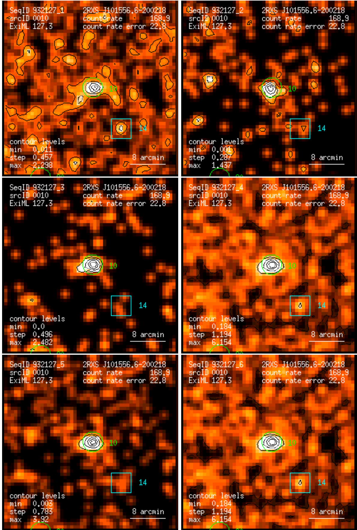
Figure 10: RASS 932127: detection 0010: band rate images, Gaussian filter: (1) PSPC channels 11 – 41, (2) 52 – 90, (3) 91 – 201, (4) 11 – 235, (5) 52 – 201, (6) 11 – 201. Broad band rates in counts/ks. Band rate contour levels in counts/ks/arcmin 2 .
