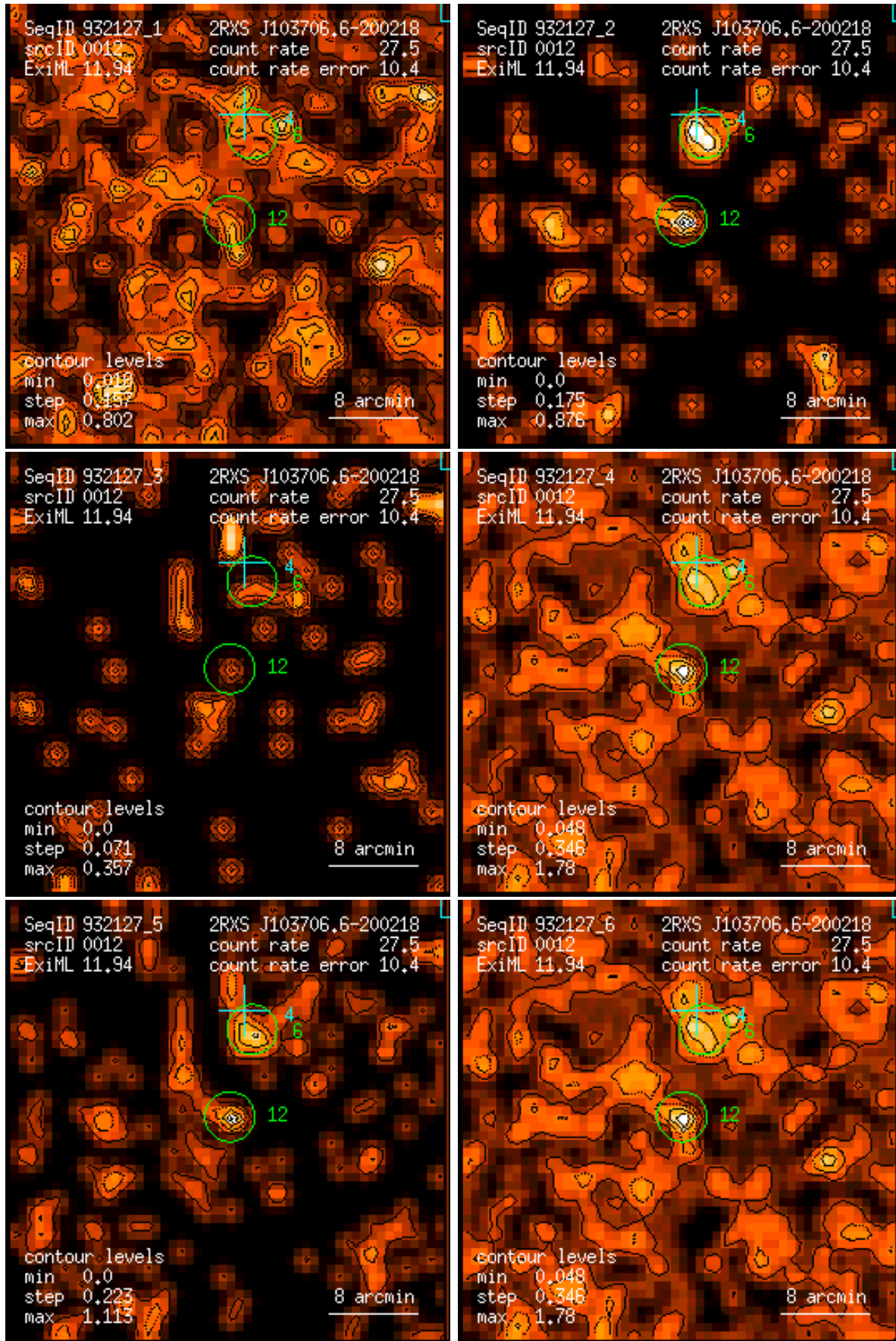
Figure 12: RASS 932127: detection 0012: band rate images, Gaussian filter: (1) PSPC channels 11 – 41, (2) 52 – 90, (3) 91 – 201, (4) 11 – 235, (5) 52 – 201, (6) 11 – 201. Broad band rates in counts/ks. Band rate contour levels in counts/ks/arcmin 2 .
