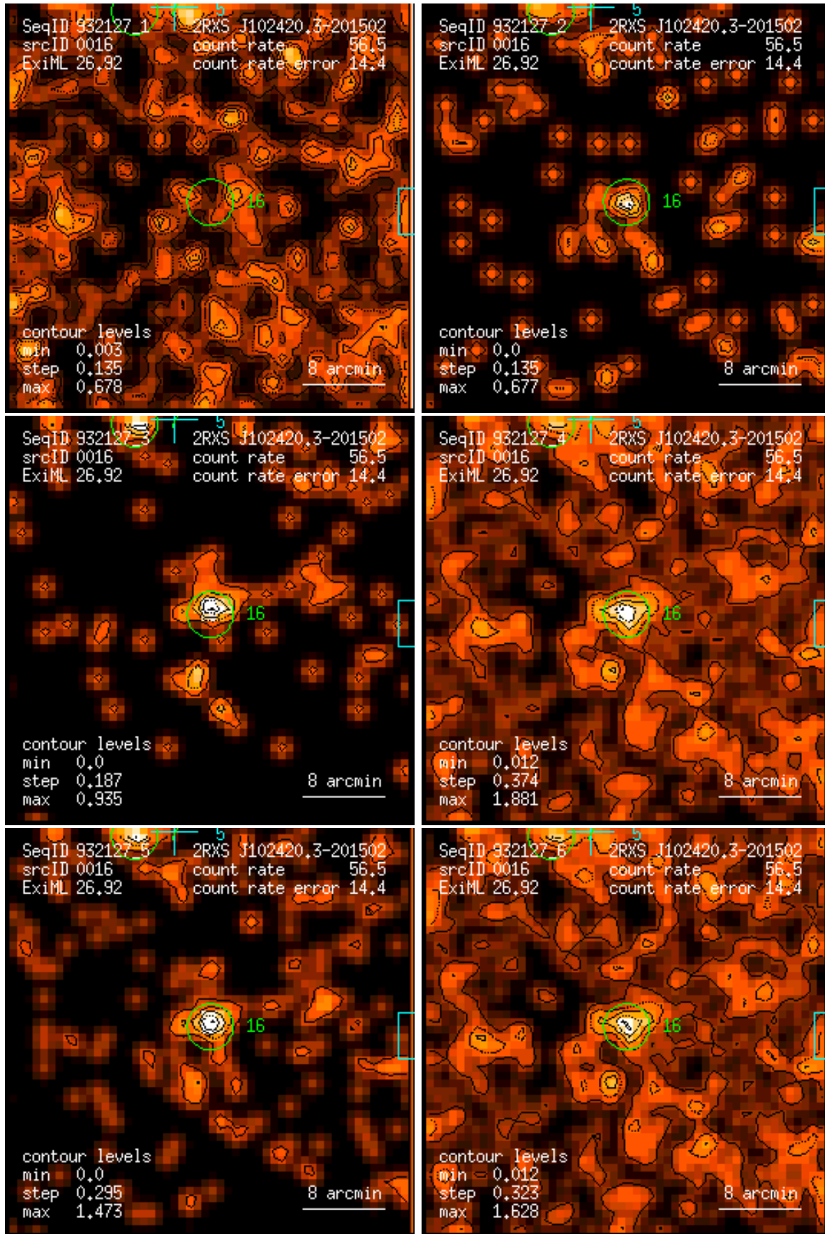
Figure 16: RASS 932127: detection 0016: band rate images, Gaussian filter: (1) PSPC channels 11 – 41, (2) 52 – 90, (3) 91 – 201, (4) 11 – 235, (5) 52 – 201, (6) 11 – 201. Broad band rates in counts/ks. Band rate contour levels in counts/ks/arcmin 2 .
