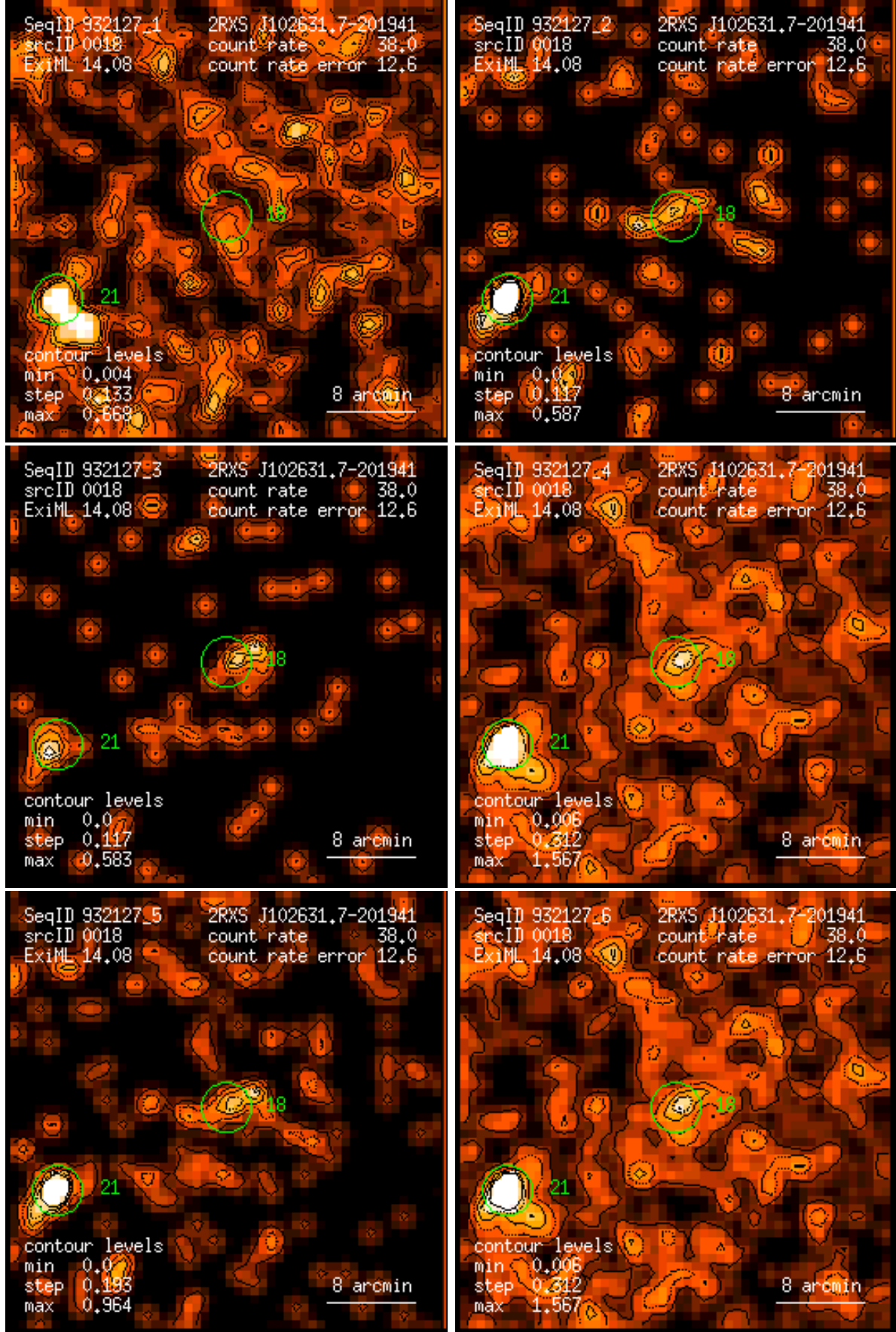
Figure 18: RASS 932127: detection 0018: band rate images, Gaussian filter: (1) PSPC channels 11 – 41, (2) 52 – 90, (3) 91 – 201, (4) 11 – 235, (5) 52 – 201, (6) 11 – 201. Broad band rates in counts/ks. Band rate contour levels in counts/ks/arcmin 2 .
