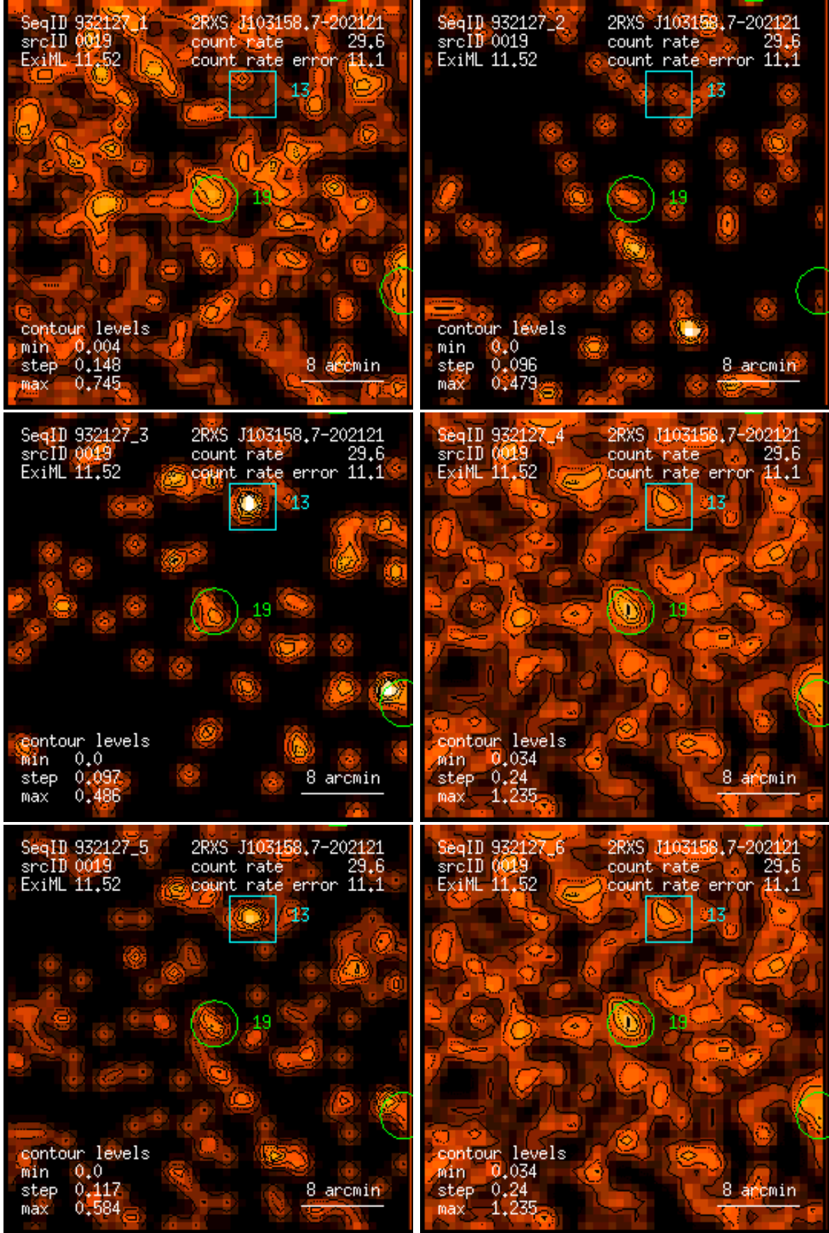
Figure 19: RASS 932127: detection 0019: band rate images, Gaussian filter: (1) PSPC channels 11 – 41, (2) 52 – 90, (3) 91 – 201, (4) 11 – 235, (5) 52 – 201, (6) 11 – 201. Broad band rates in counts/ks. Band rate contour levels in counts/ks/arcmin 2 .
