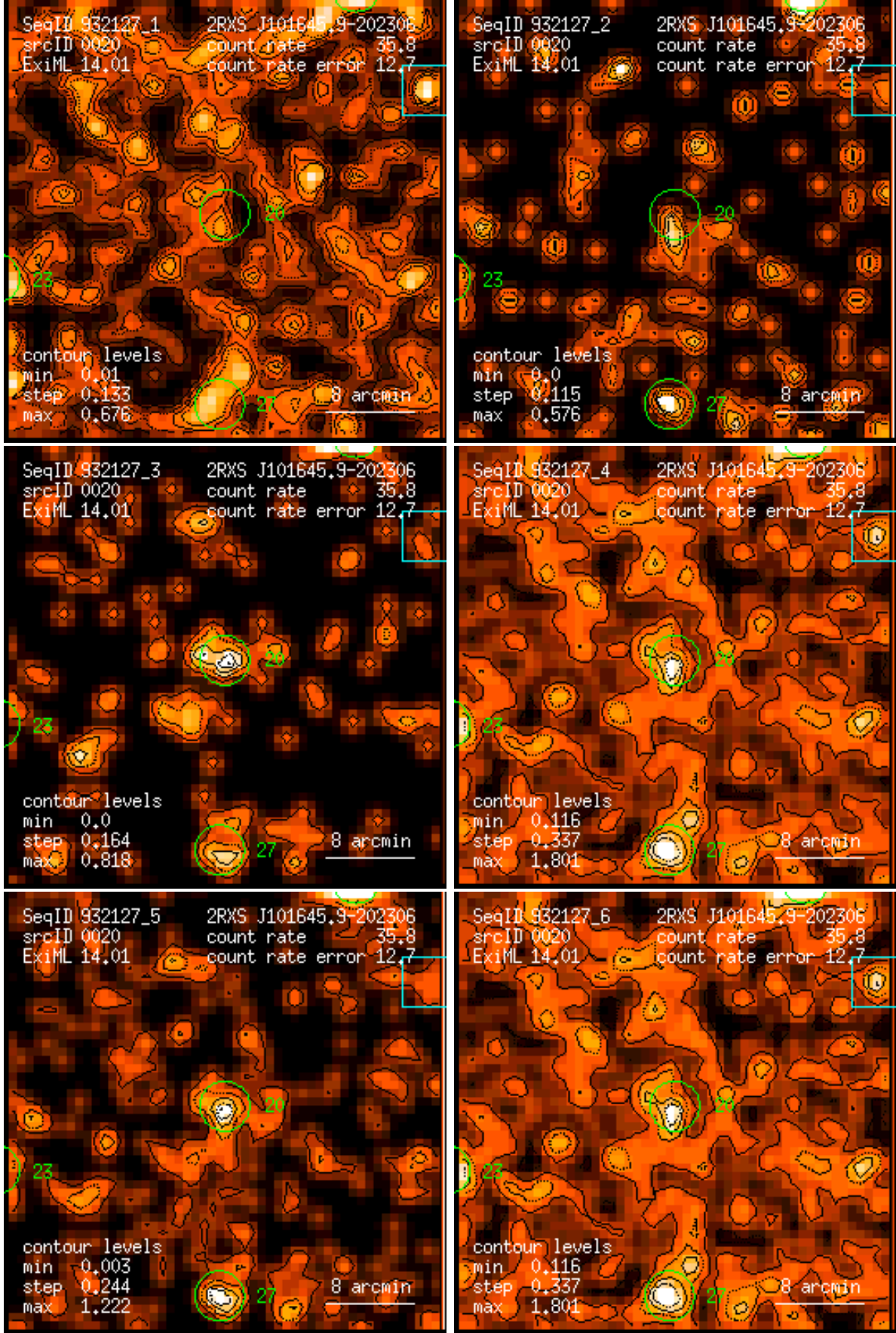
Figure 20: RASS 932127: detection 0020: band rate images, Gaussian filter: (1) PSPC channels 11 – 41, (2) 52 – 90, (3) 91 – 201, (4) 11 – 235, (5) 52 – 201, (6) 11 – 201. Broad band rates in counts/ks. Band rate contour levels in counts/ks/arcmin 2 .
