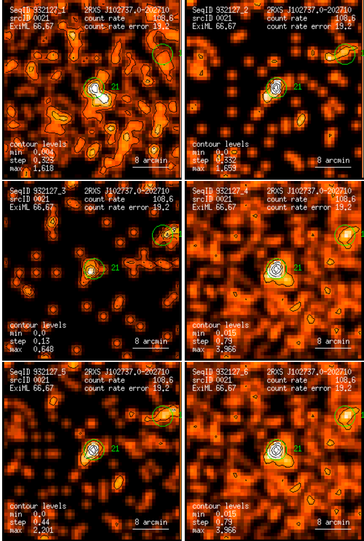
Figure 21: RASS 932127: detection 0021: band rate images, Gaussian filter: (1) PSPC channels 11 – 41, (2) 52 – 90, (3) 91 – 201, (4) 11 – 235, (5) 52 – 201, (6) 11 – 201. Broad band rates in counts/ks. Band rate contour levels in counts/ks/arcmin 2 .
