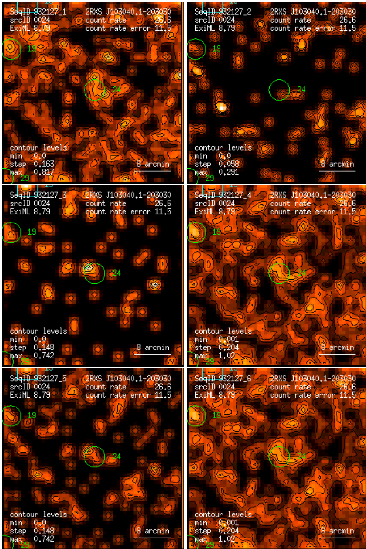
Figure 24: RASS 932127: detection 0024: band rate images, Gaussian filter: (1) PSPC channels 11 – 41, (2) 52 – 90, (3) 91 – 201, (4) 11 – 235, (5) 52 – 201, (6) 11 – 201. Broad band rates in counts/ks. Band rate contour levels in counts/ks/arcmin 2 .
