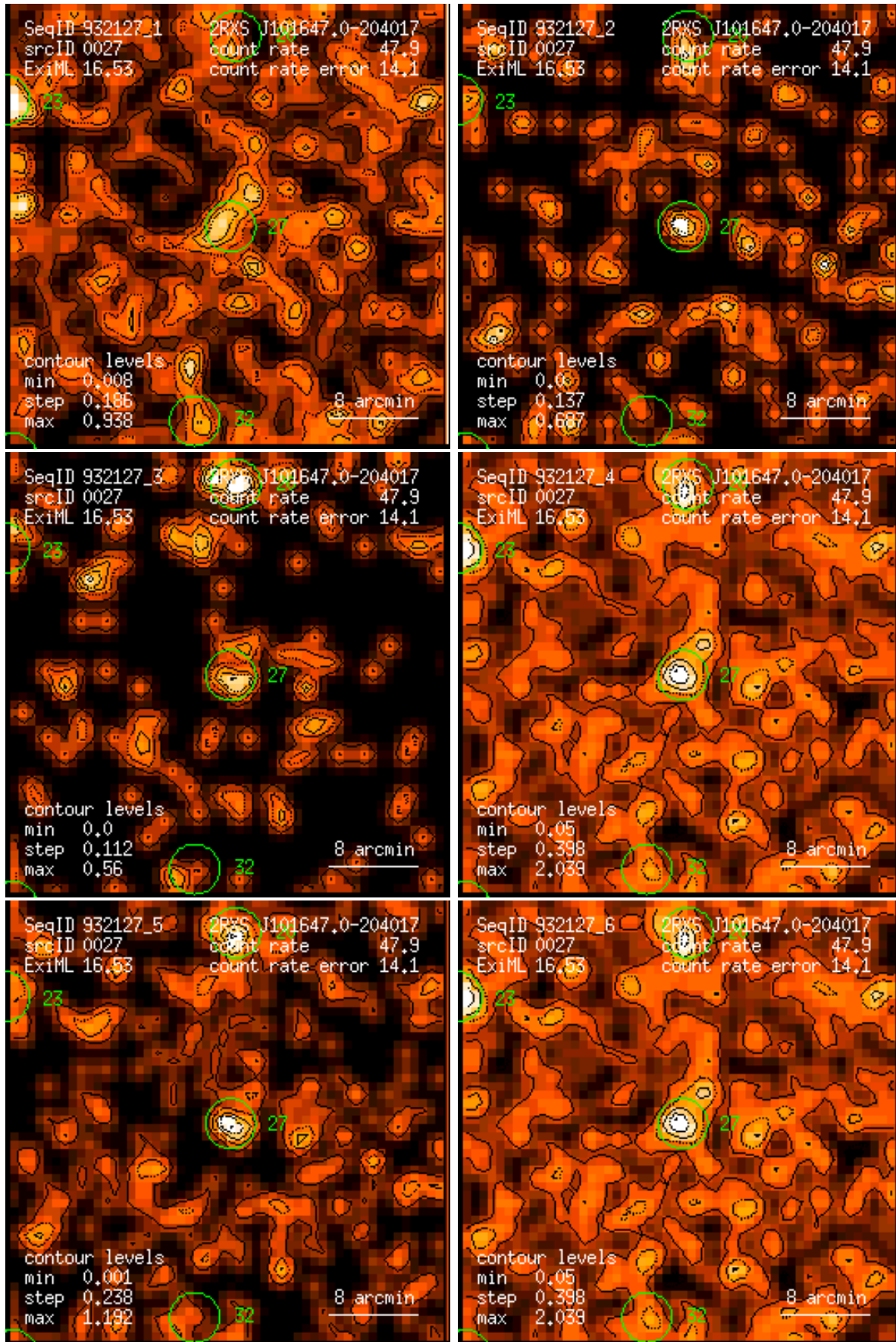
Figure 27: RASS 932127: detection 0027: band rate images, Gaussian filter: (1) PSPC channels 11 – 41, (2) 52 – 90, (3) 91 – 201, (4) 11 – 235, (5) 52 – 201, (6) 11 – 201. Broad band rates in counts/ks. Band rate contour levels in counts/ks/arcmin 2 .
