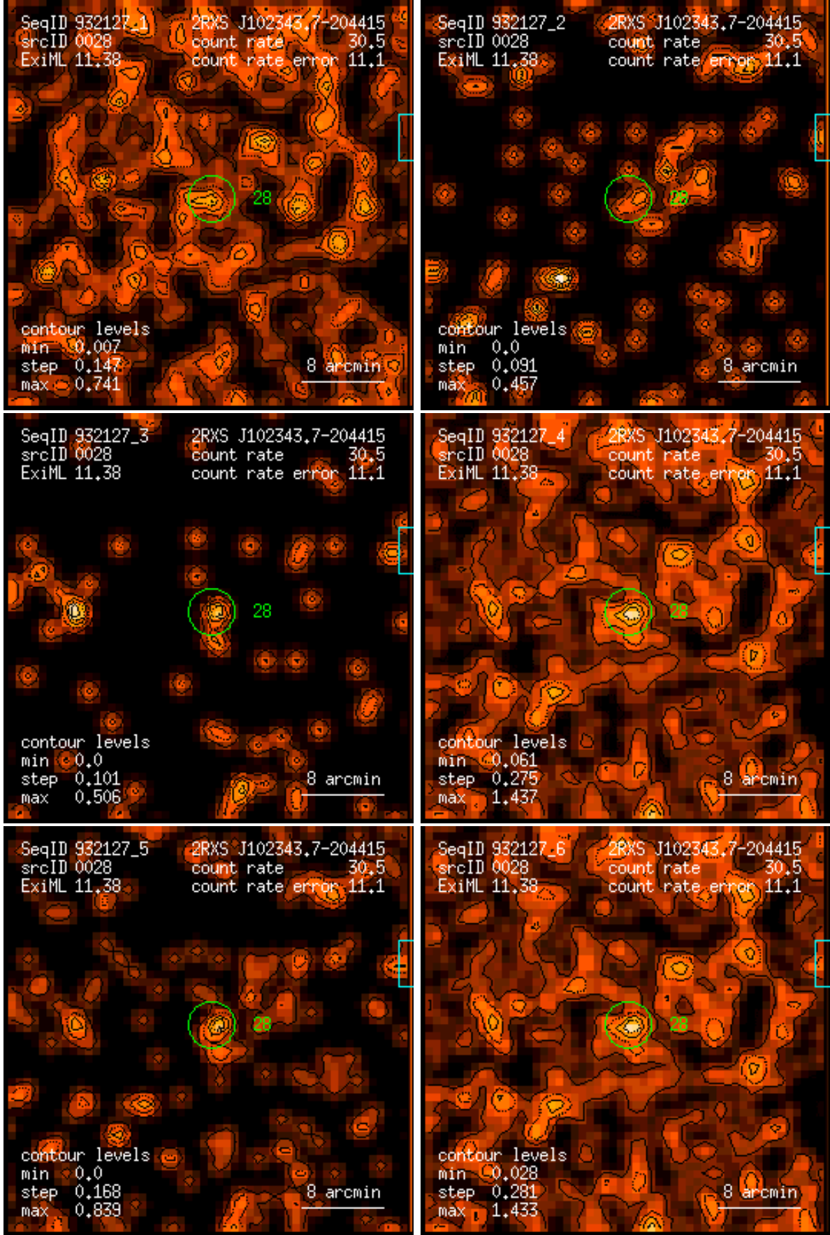
Figure 28: RASS 932127: detection 0028: band rate images, Gaussian filter: (1) PSPC channels 11 – 41, (2) 52 – 90, (3) 91 – 201, (4) 11 – 235, (5) 52 – 201, (6) 11 – 201. Broad band rates in counts/ks. Band rate contour levels in counts/ks/arcmin 2 .
