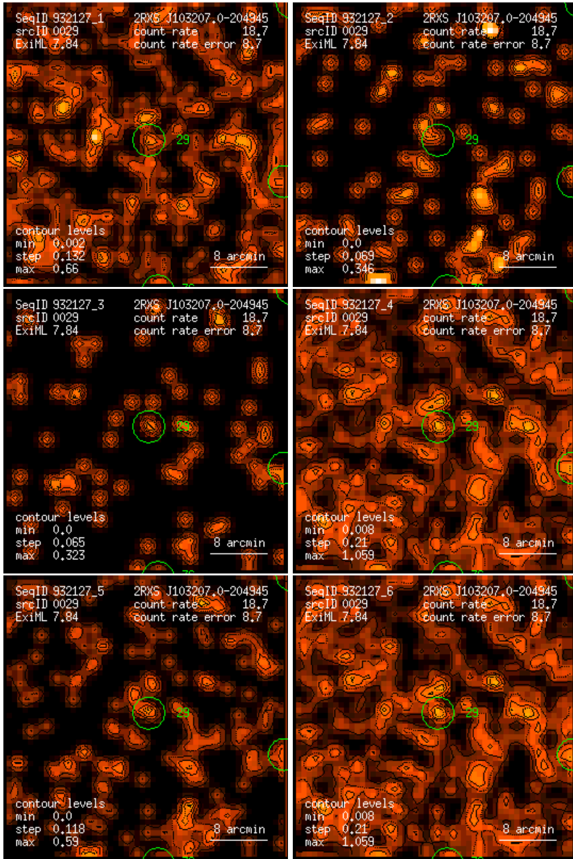
Figure 29: RASS 932127: detection 0029: band rate images, Gaussian filter: (1) PSPC channels 11 – 41, (2) 52 – 90, (3) 91 – 201, (4) 11 – 235, (5) 52 – 201, (6) 11 – 201. Broad band rates in counts/ks. Band rate contour levels in counts/ks/arcmin 2 .
