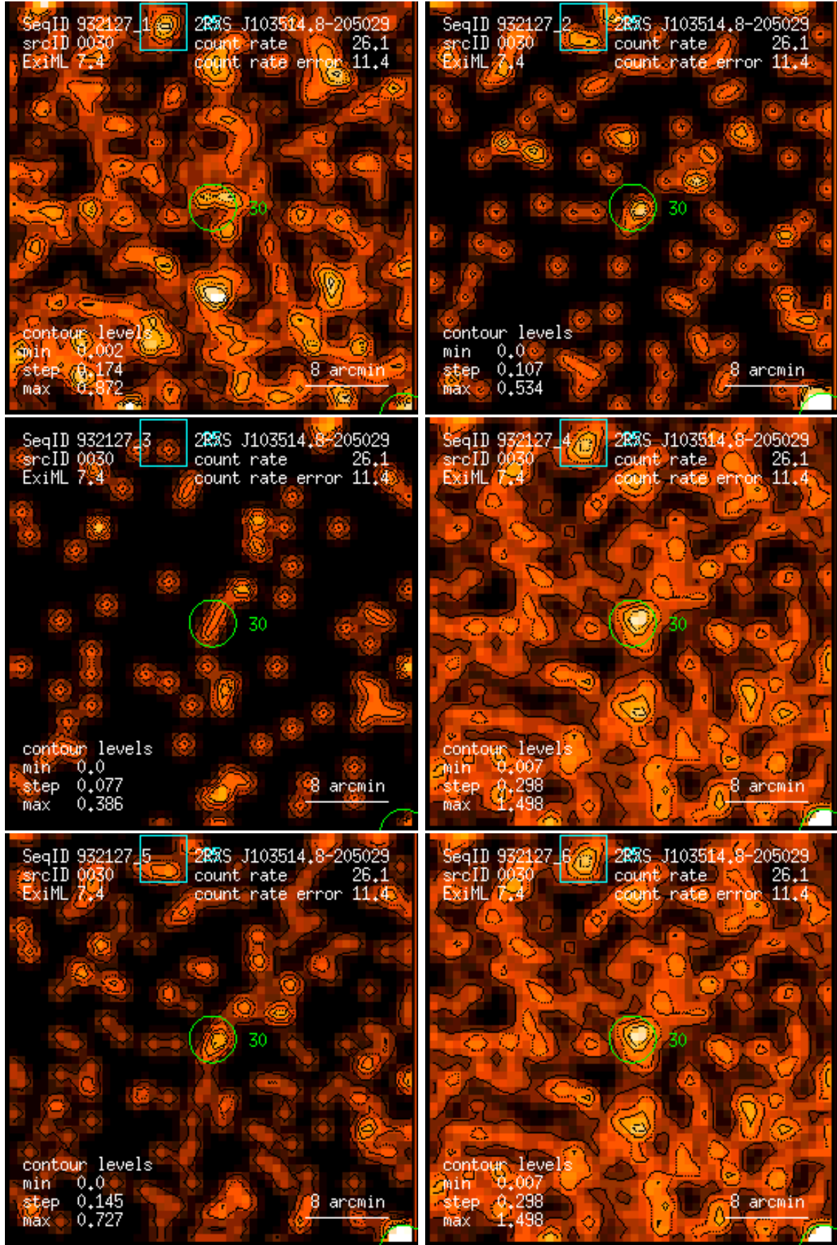
Figure 30: RASS 932127: detection 0030: band rate images, Gaussian filter: (1) PSPC channels 11 – 41, (2) 52 – 90, (3) 91 – 201, (4) 11 – 235, (5) 52 – 201, (6) 11 – 201. Broad band rates in counts/ks. Band rate contour levels in counts/ks/arcmin 2 .
