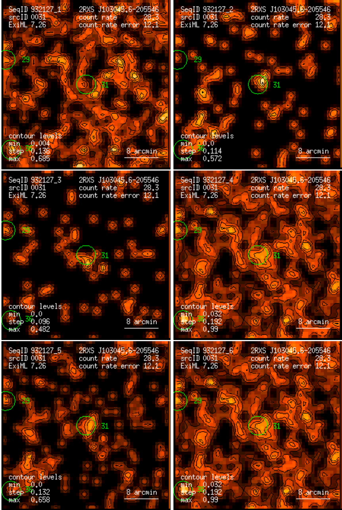
Figure 31: RASS 932127: detection 0031: band rate images, Gaussian filter: (1) PSPC channels 11 – 41, (2) 52 – 90, (3) 91 – 201, (4) 11 – 235, (5) 52 – 201, (6) 11 – 201. Broad band rates in counts/ks. Band rate contour levels in counts/ks/arcmin 2 .
