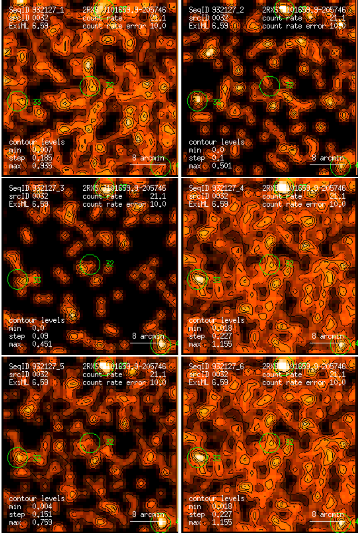
Figure 32: RASS 932127: detection 0032: band rate images, Gaussian filter: (1) PSPC channels 11 – 41, (2) 52 – 90, (3) 91 – 201, (4) 11 – 235, (5) 52 – 201, (6) 11 – 201. Broad band rates in counts/ks. Band rate contour levels in counts/ks/arcmin 2 .
