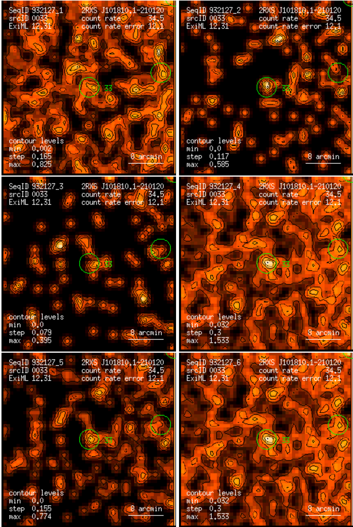
Figure 33: RASS 932127: detection 0033: band rate images, Gaussian filter: (1) PSPC channels 11 – 41, (2) 52 – 90, (3) 91 – 201, (4) 11 – 235, (5) 52 – 201, (6) 11 – 201. Broad band rates in counts/ks. Band rate contour levels in counts/ks/arcmin 2 .
