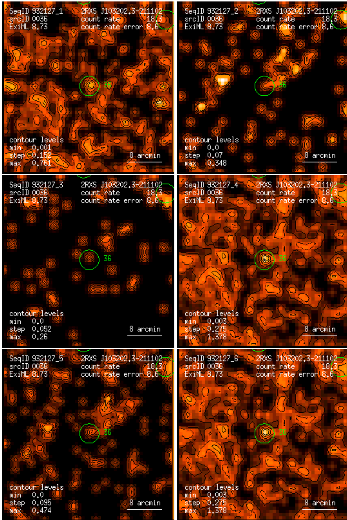
Figure 36: RASS 932127: detection 0036: band rate images, Gaussian filter: (1) PSPC channels 11 – 41, (2) 52 – 90, (3) 91 – 201, (4) 11 – 235, (5) 52 – 201, (6) 11 – 201. Broad band rates in counts/ks. Band rate contour levels in counts/ks/arcmin 2 .
