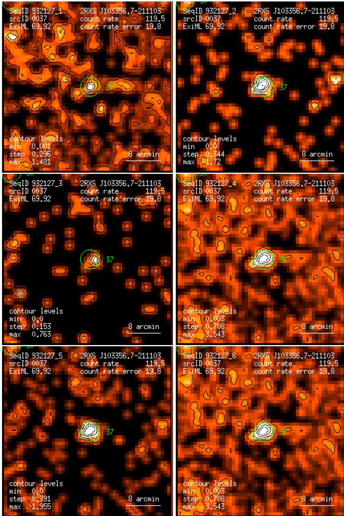
Figure 37: RASS 932127: detection 0037: band rate images, Gaussian filter: (1) PSPC channels 11 – 41, (2) 52 – 90, (3) 91 – 201, (4) 11 – 235, (5) 52 – 201, (6) 11 – 201. Broad band rates in counts/ks. Band rate contour levels in counts/ks/arcmin 2 .
