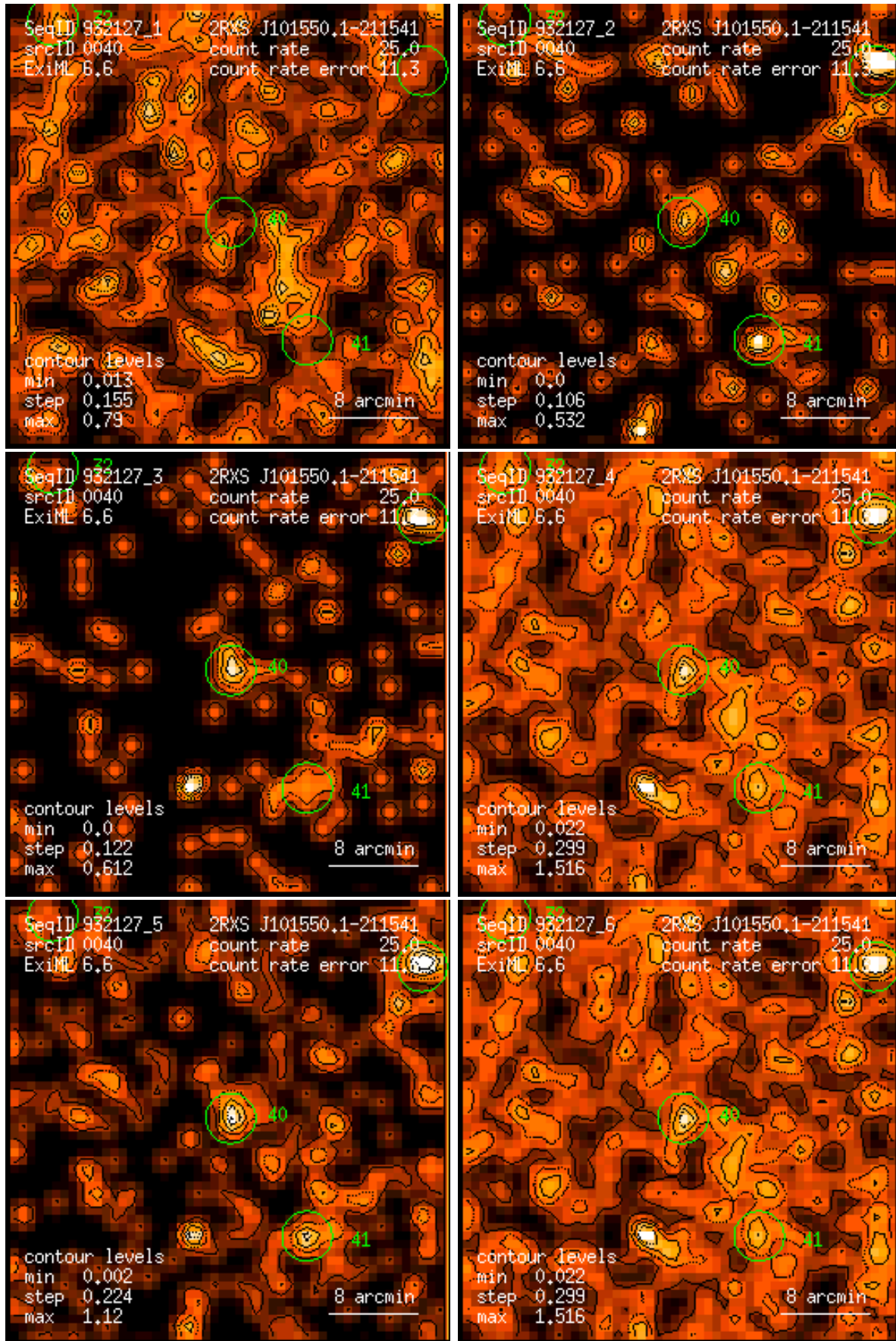
Figure 40: RASS 932127: detection 0040: band rate images, Gaussian filter: (1) PSPC channels 11 – 41, (2) 52 – 90, (3) 91 – 201, (4) 11 – 235, (5) 52 – 201, (6) 11 – 201. Broad band rates in counts/ks. Band rate contour levels in counts/ks/arcmin 2 .
