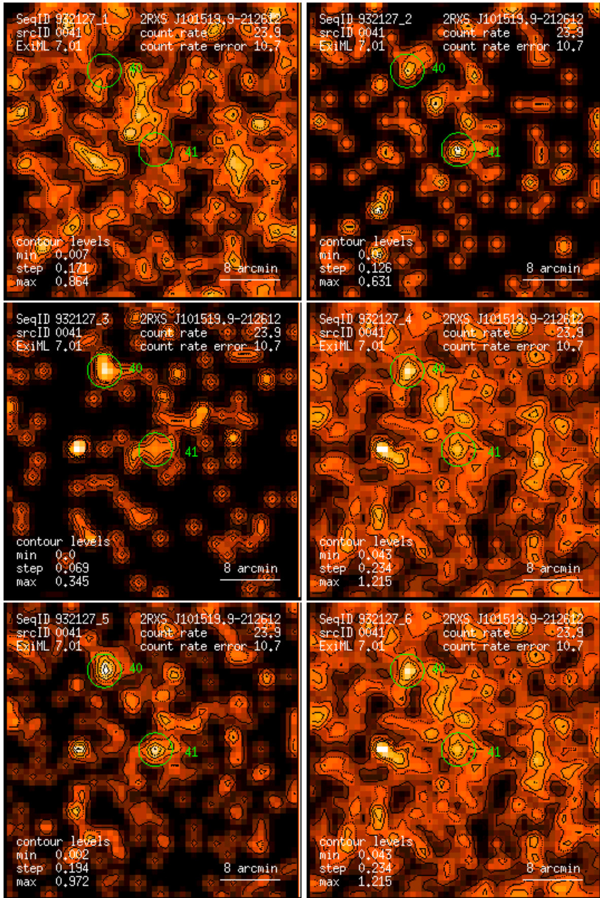
Figure 41: RASS 932127: detection 0041: band rate images, Gaussian filter: (1) PSPC channels 11 – 41, (2) 52 – 90, (3) 91 – 201, (4) 11 – 235, (5) 52 – 201, (6) 11 – 201. Broad band rates in counts/ks. Band rate contour levels in counts/ks/arcmin 2 .
