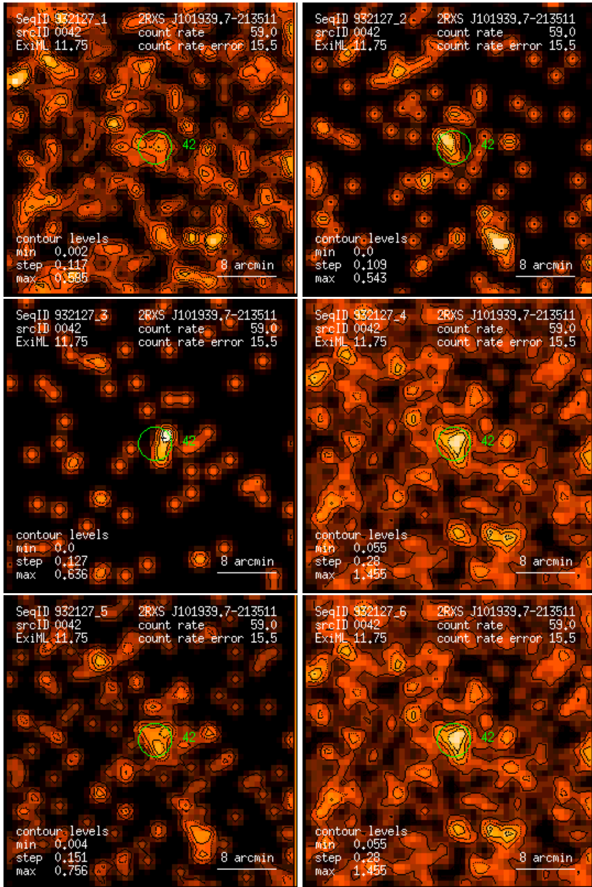
Figure 42: RASS 932127: detection 0042: band rate images, Gaussian filter: (1) PSPC channels 11 – 41, (2) 52 – 90, (3) 91 – 201, (4) 11 – 235, (5) 52 – 201, (6) 11 – 201. Broad band rates in counts/ks. Band rate contour levels in counts/ks/arcmin 2 .
