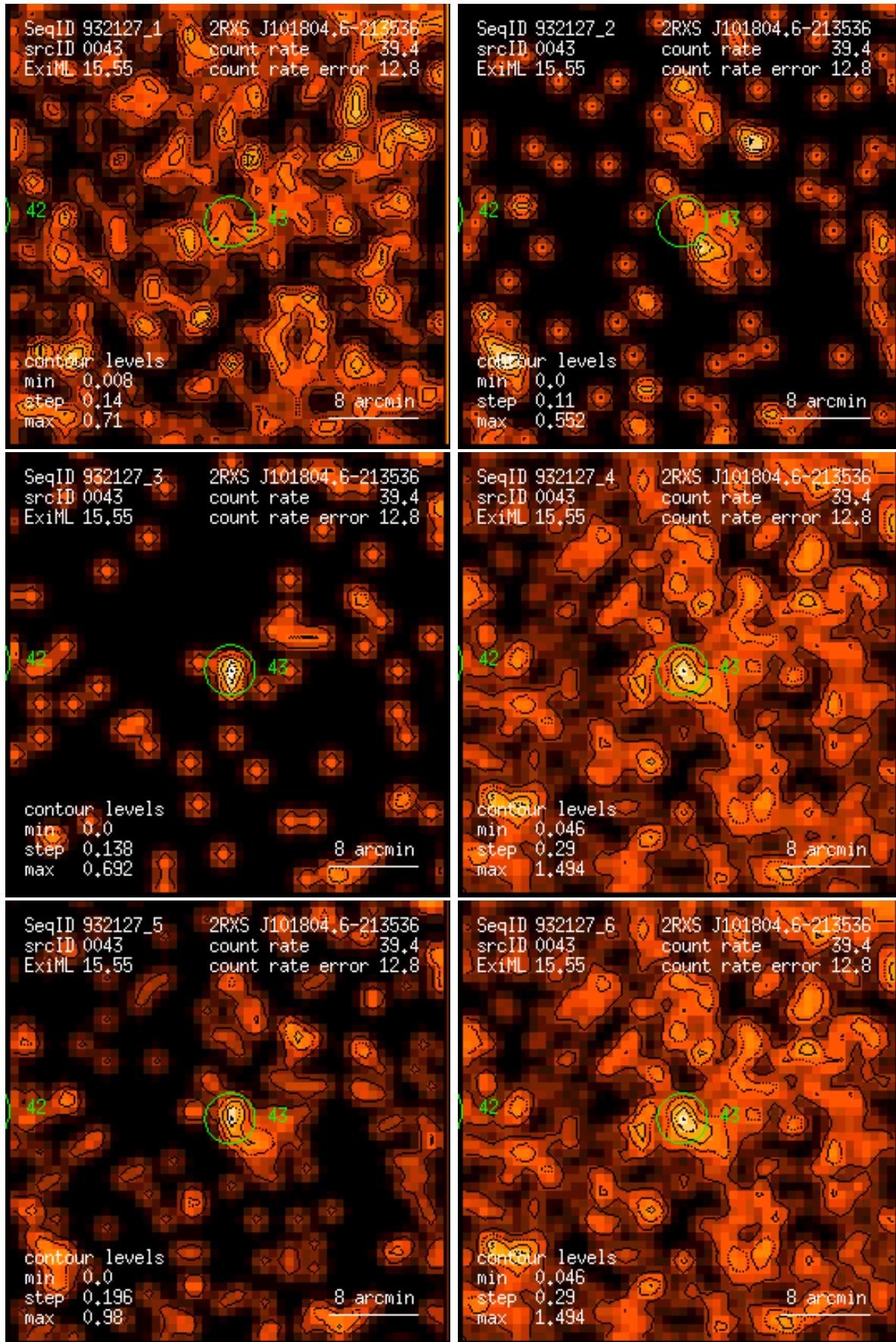
Figure 43: RASS 932127: detection 0043: band rate images, Gaussian filter: (1) PSPC channels 11 – 41, (2) 52 – 90, (3) 91 – 201, (4) 11 – 235, (5) 52 – 201, (6) 11 – 201. Broad band rates in counts/ks. Band rate contour levels in counts/ks/arcmin 2 .
