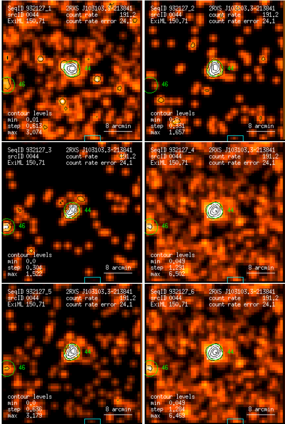
Figure 44: RASS 932127: detection 0044: band rate images, Gaussian filter: (1) PSPC channels 11 – 41, (2) 52 – 90, (3) 91 – 201, (4) 11 – 235, (5) 52 – 201, (6) 11 – 201. Broad band rates in counts/ks. Band rate contour levels in counts/ks/arcmin 2 .
