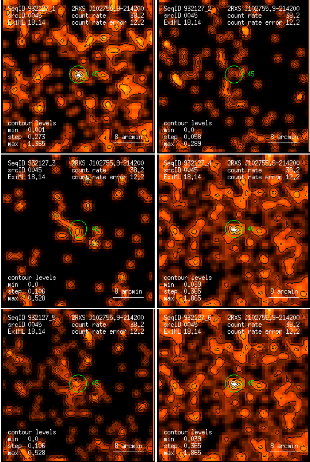
Figure 45: RASS 932127: detection 0045: band rate images, Gaussian filter: (1) PSPC channels 11 – 41, (2) 52 – 90, (3) 91 – 201, (4) 11 – 235, (5) 52 – 201, (6) 11 – 201. Broad band rates in counts/ks. Band rate contour levels in counts/ks/arcmin 2 .
