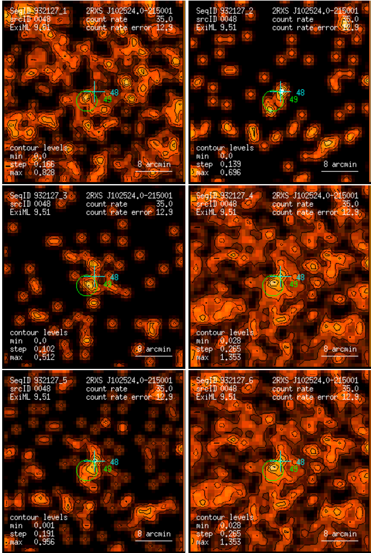
Figure 48: RASS 932127: detection 0048: band rate images, Gaussian filter: (1) PSPC channels 11 – 41, (2) 52 – 90, (3) 91 – 201, (4) 11 – 235, (5) 52 – 201, (6) 11 – 201. Broad band rates in counts/ks. Band rate contour levels in counts/ks/arcmin 2 .
