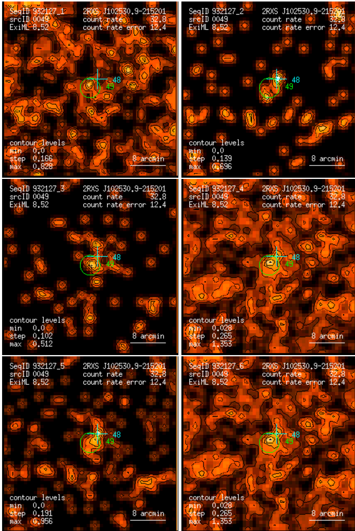
Figure 49: RASS 932127: detection 0049: band rate images, Gaussian filter: (1) PSPC channels 11 – 41, (2) 52 – 90, (3) 91 – 201, (4) 11 – 235, (5) 52 – 201, (6) 11 – 201. Broad band rates in counts/ks. Band rate contour levels in counts/ks/arcmin 2 .
