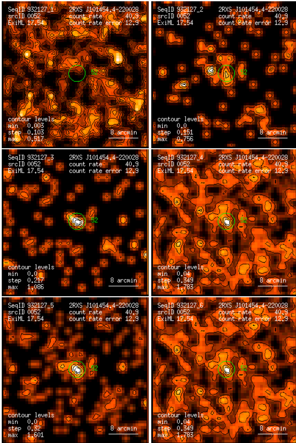
Figure 52: RASS 932127: detection 0052: band rate images, Gaussian filter: (1) PSPC channels 11 – 41, (2) 52 – 90, (3) 91 – 201, (4) 11 – 235, (5) 52 – 201, (6) 11 – 201. Broad band rates in counts/ks. Band rate contour levels in counts/ks/arcmin 2 .
