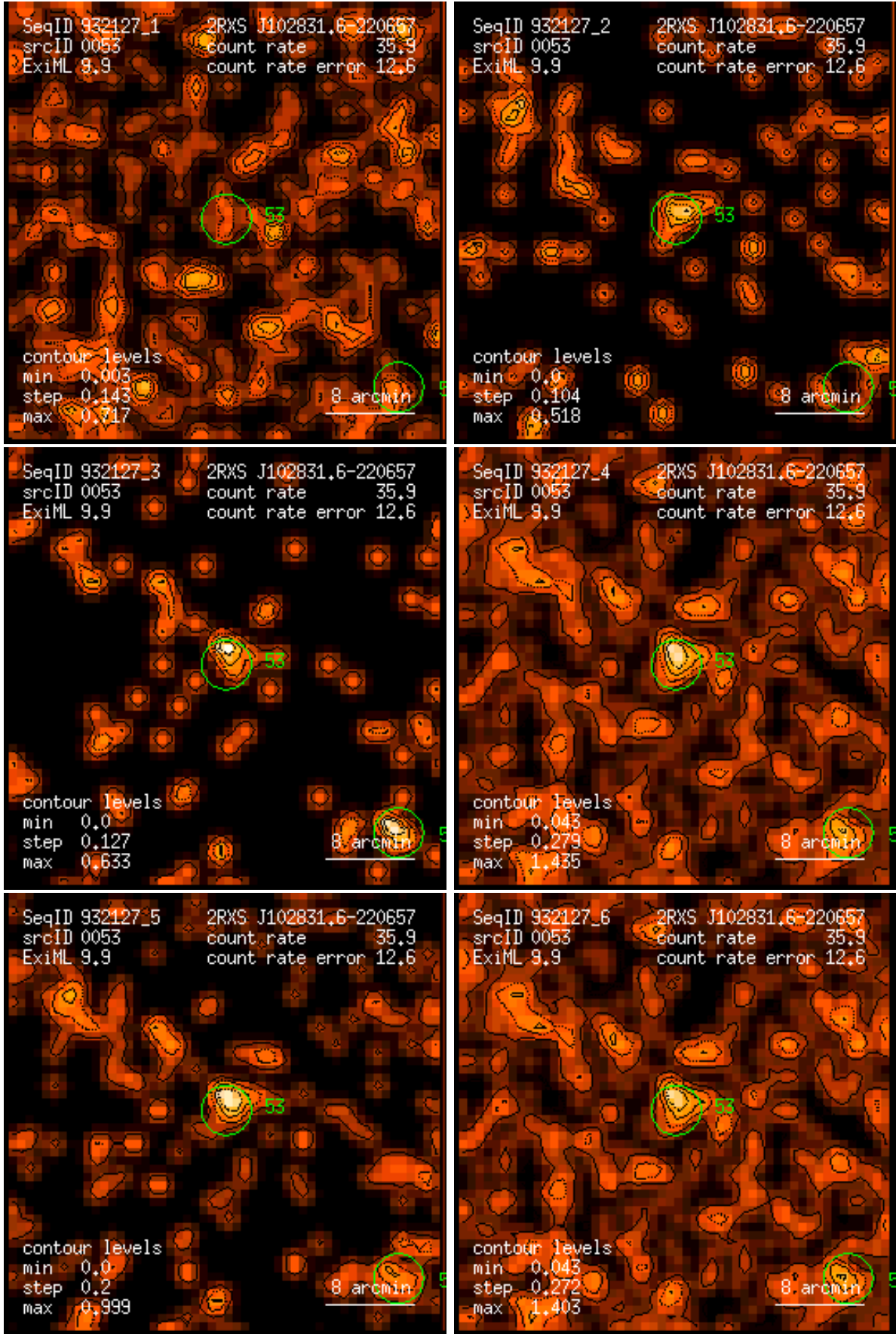
Figure 53: RASS 932127: detection 0053: band rate images, Gaussian filter: (1) PSPC channels 11 – 41, (2) 52 – 90, (3) 91 – 201, (4) 11 – 235, (5) 52 – 201, (6) 11 – 201. Broad band rates in counts/ks. Band rate contour levels in counts/ks/arcmin 2 .
