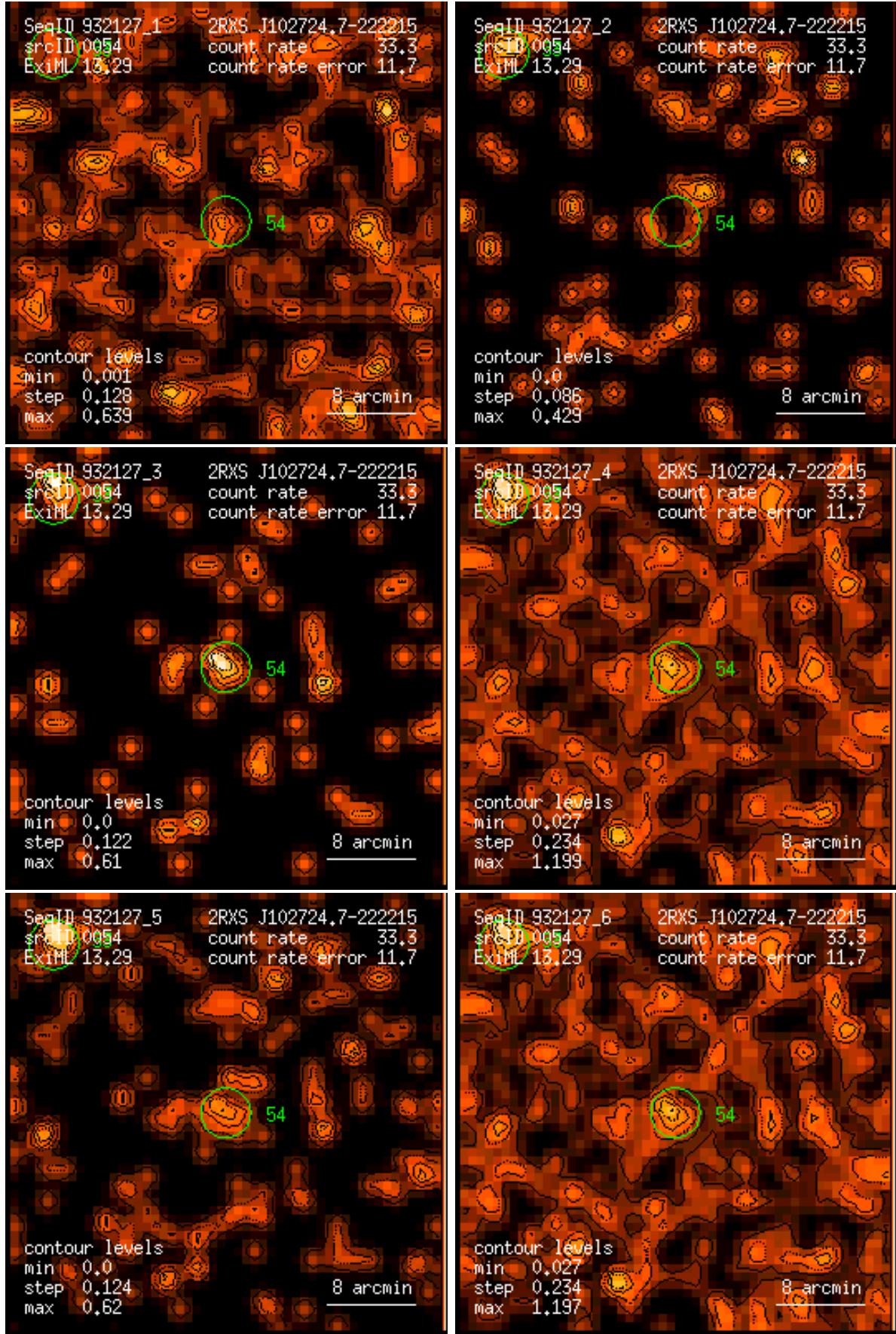
Figure 54: RASS 932127: detection 0054: band rate images, Gaussian filter: (1) PSPC channels 11 – 41, (2) 52 – 90, (3) 91 – 201, (4) 11 – 235, (5) 52 – 201, (6) 11 – 201. Broad band rates in counts/ks. Band rate contour levels in counts/ks/arcmin 2 .
