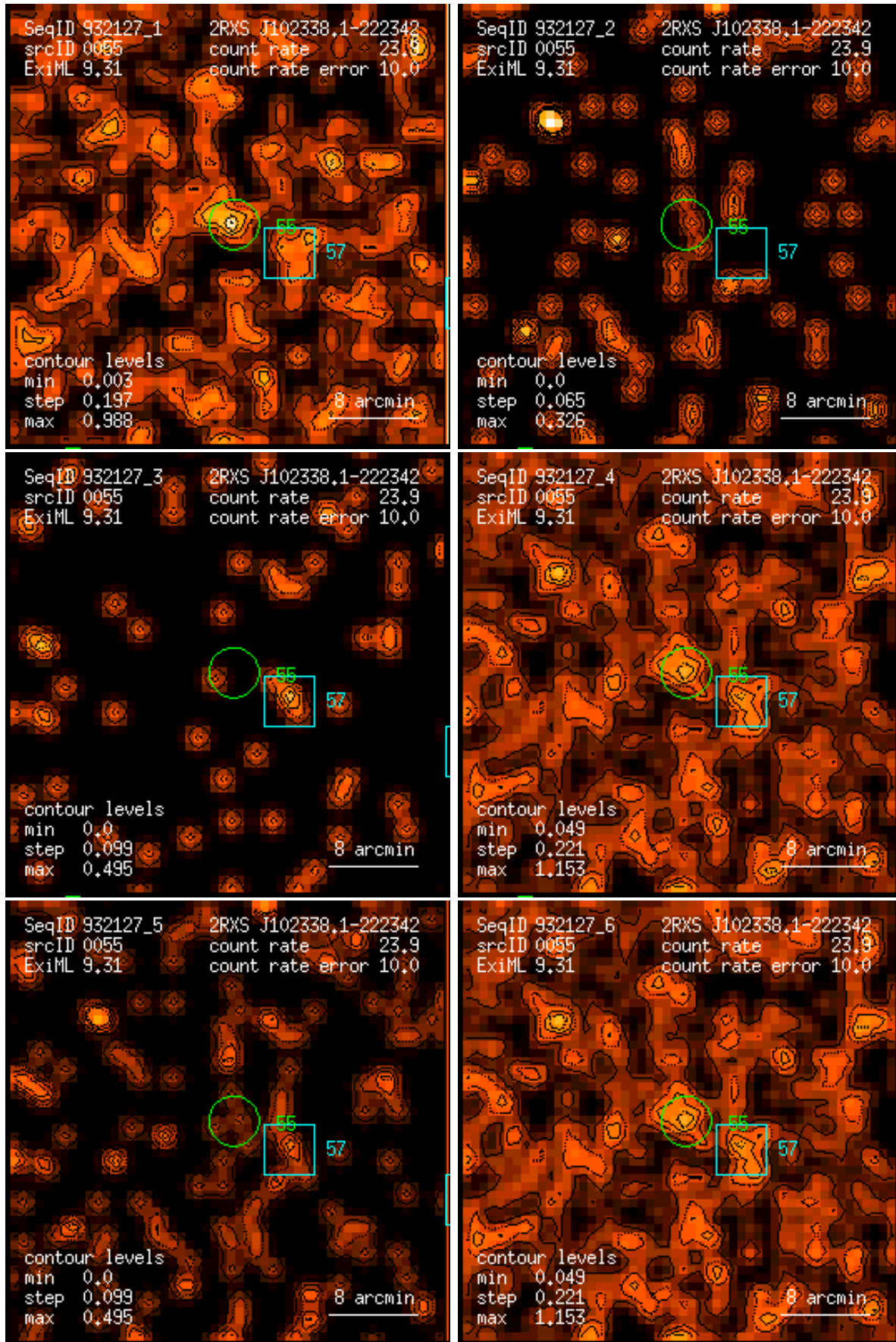
Figure 55: RASS 932127: detection 0055: band rate images, Gaussian filter: (1) PSPC channels 11 – 41, (2) 52 – 90, (3) 91 – 201, (4) 11 – 235, (5) 52 – 201, (6) 11 – 201. Broad band rates in counts/ks. Band rate contour levels in counts/ks/arcmin 2 .
