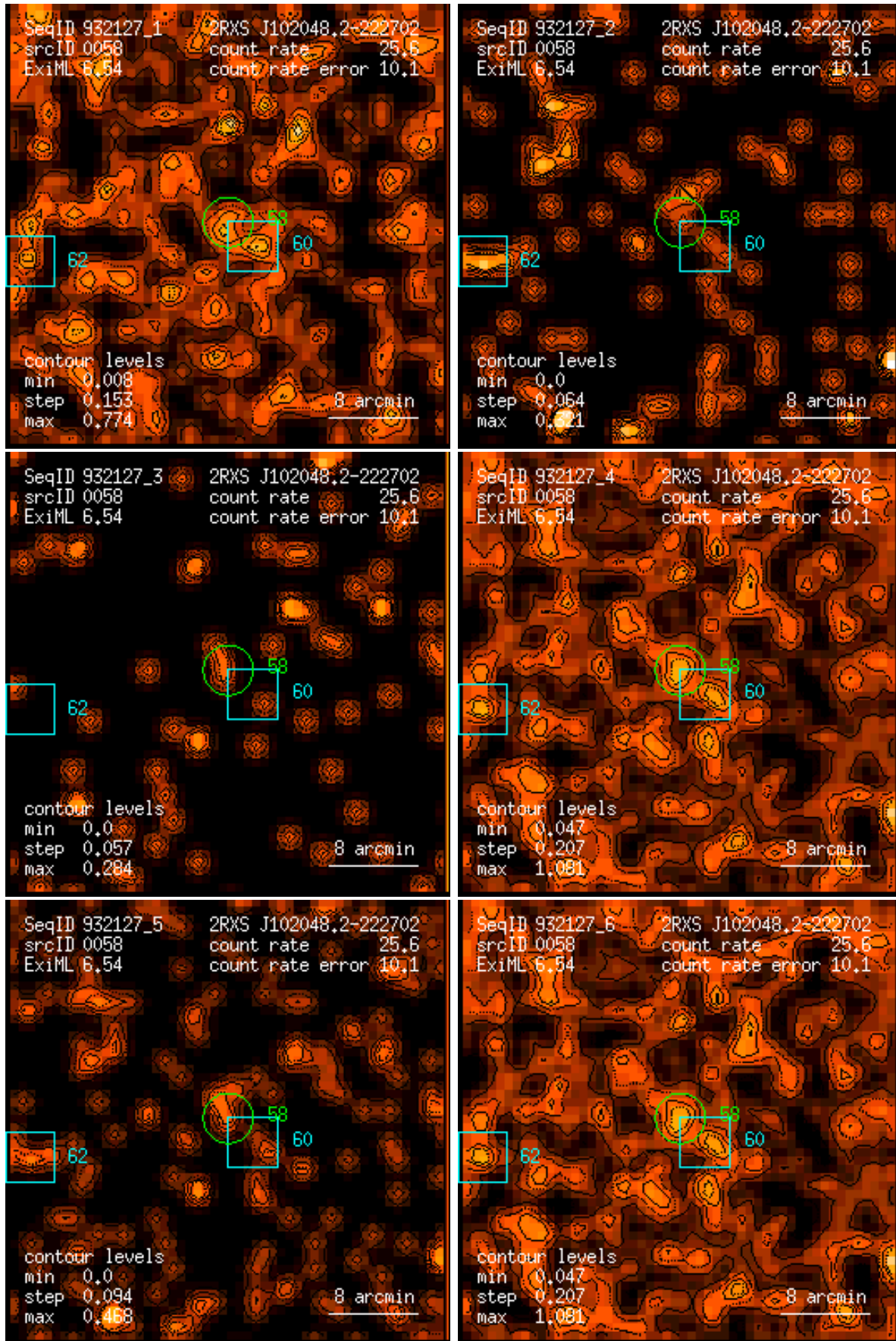
Figure 58: RASS 932127: detection 0058: band rate images, Gaussian filter: (1) PSPC channels 11 – 41, (2) 52 – 90, (3) 91 – 201, (4) 11 – 235, (5) 52 – 201, (6) 11 – 201. Broad band rates in counts/ks. Band rate contour levels in counts/ks/arcmin 2 .
