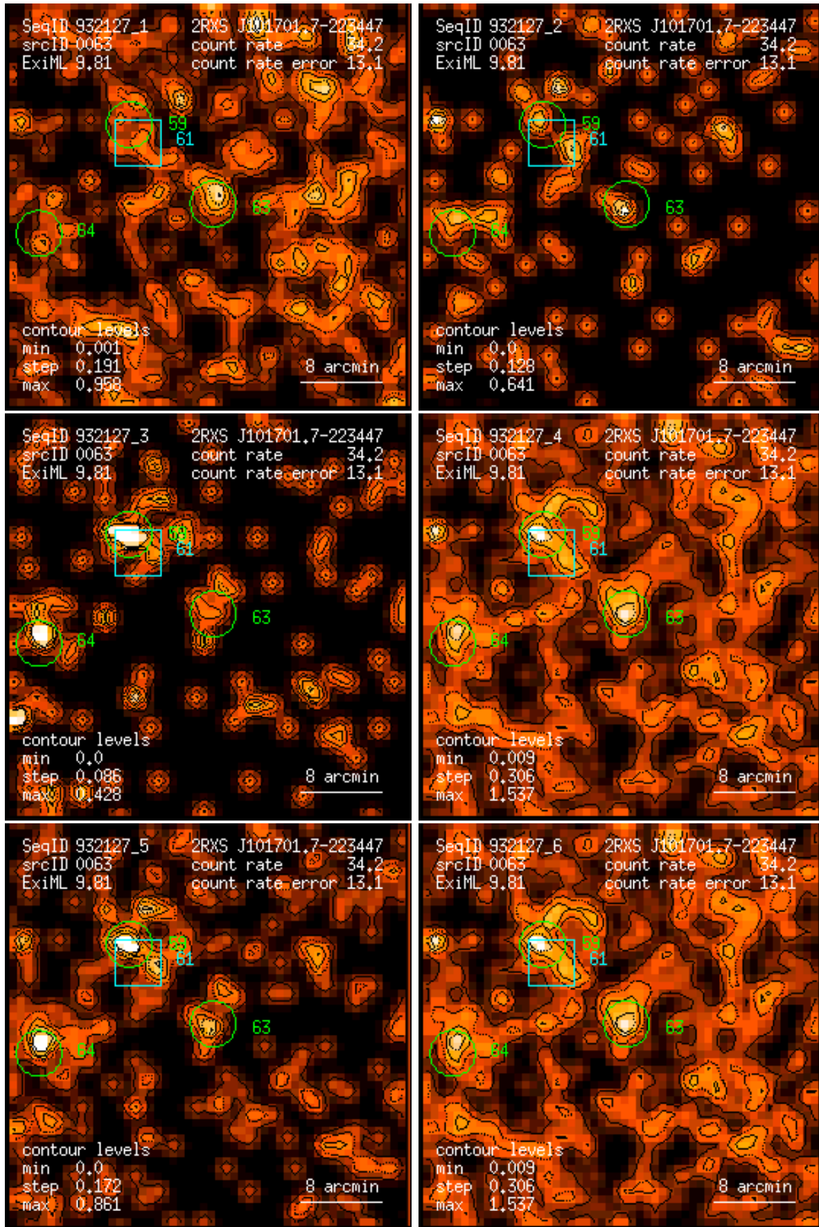
Figure 63: RASS 932127: detection 0063: band rate images, Gaussian filter: (1) PSPC channels 11 – 41, (2) 52 – 90, (3) 91 – 201, (4) 11 – 235, (5) 52 – 201, (6) 11 – 201. Broad band rates in counts/ks. Band rate contour levels in counts/ks/arcmin 2 .
