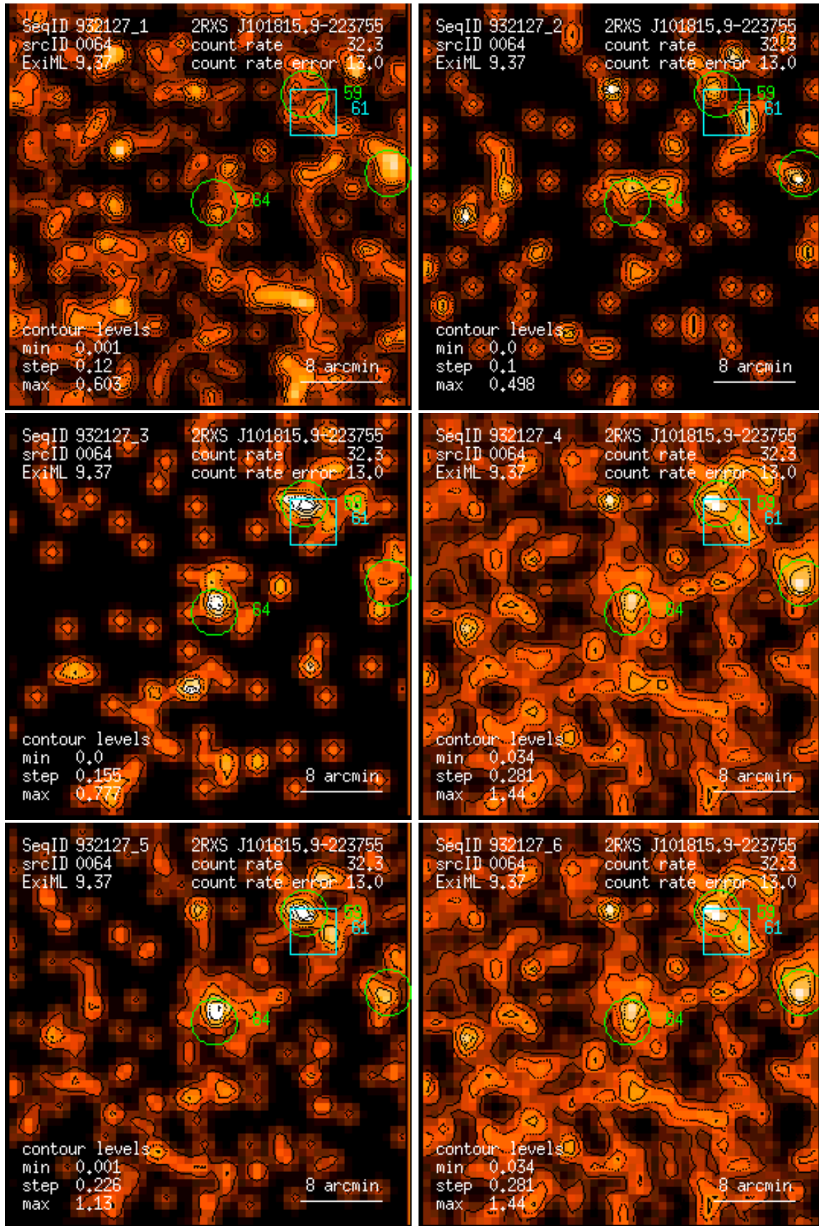
Figure 64: RASS 932127: detection 0064: band rate images, Gaussian filter: (1) PSPC channels 11 – 41, (2) 52 – 90, (3) 91 – 201, (4) 11 – 235, (5) 52 – 201, (6) 11 – 201. Broad band rates in counts/ks. Band rate contour levels in counts/ks/arcmin 2 .
