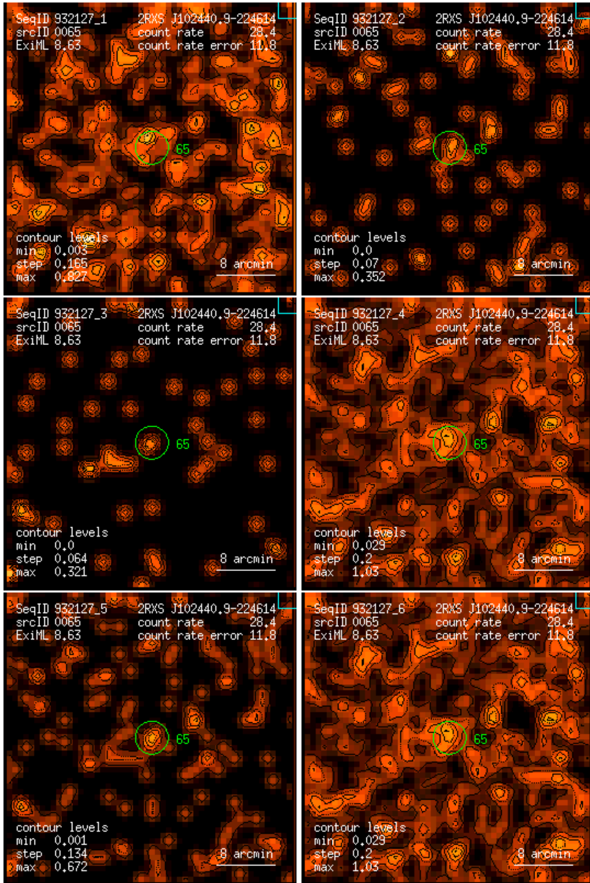
Figure 65: RASS 932127: detection 0065: band rate images, Gaussian filter: (1) PSPC channels 11 – 41, (2) 52 – 90, (3) 91 – 201, (4) 11 – 235, (5) 52 – 201, (6) 11 – 201. Broad band rates in counts/ks. Band rate contour levels in counts/ks/arcmin 2 .
