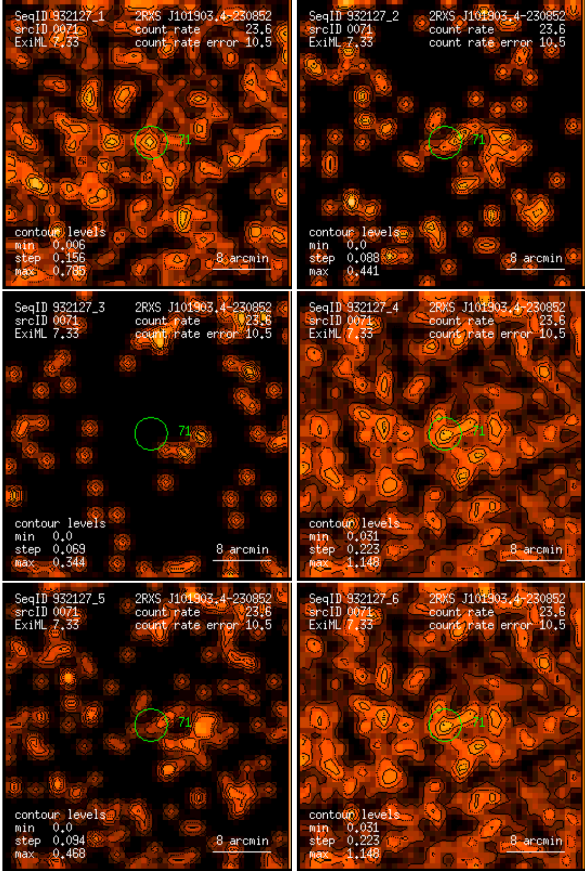
Figure 71: RASS 932127: detection 0071: band rate images, Gaussian filter: (1) PSPC channels 11 – 41, (2) 52 – 90, (3) 91 – 201, (4) 11 – 235, (5) 52 – 201, (6) 11 – 201. Broad band rates in counts/ks. Band rate contour levels in counts/ks/arcmin 2 .
