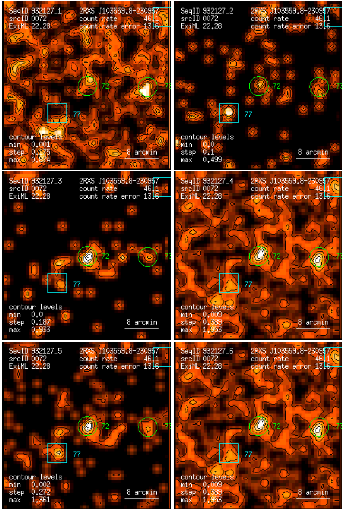
Figure 72: RASS 932127: detection 0072: band rate images, Gaussian filter: (1) PSPC channels 11 – 41, (2) 52 – 90, (3) 91 – 201, (4) 11 – 235, (5) 52 – 201, (6) 11 – 201. Broad band rates in counts/ks. Band rate contour levels in counts/ks/arcmin 2 .
