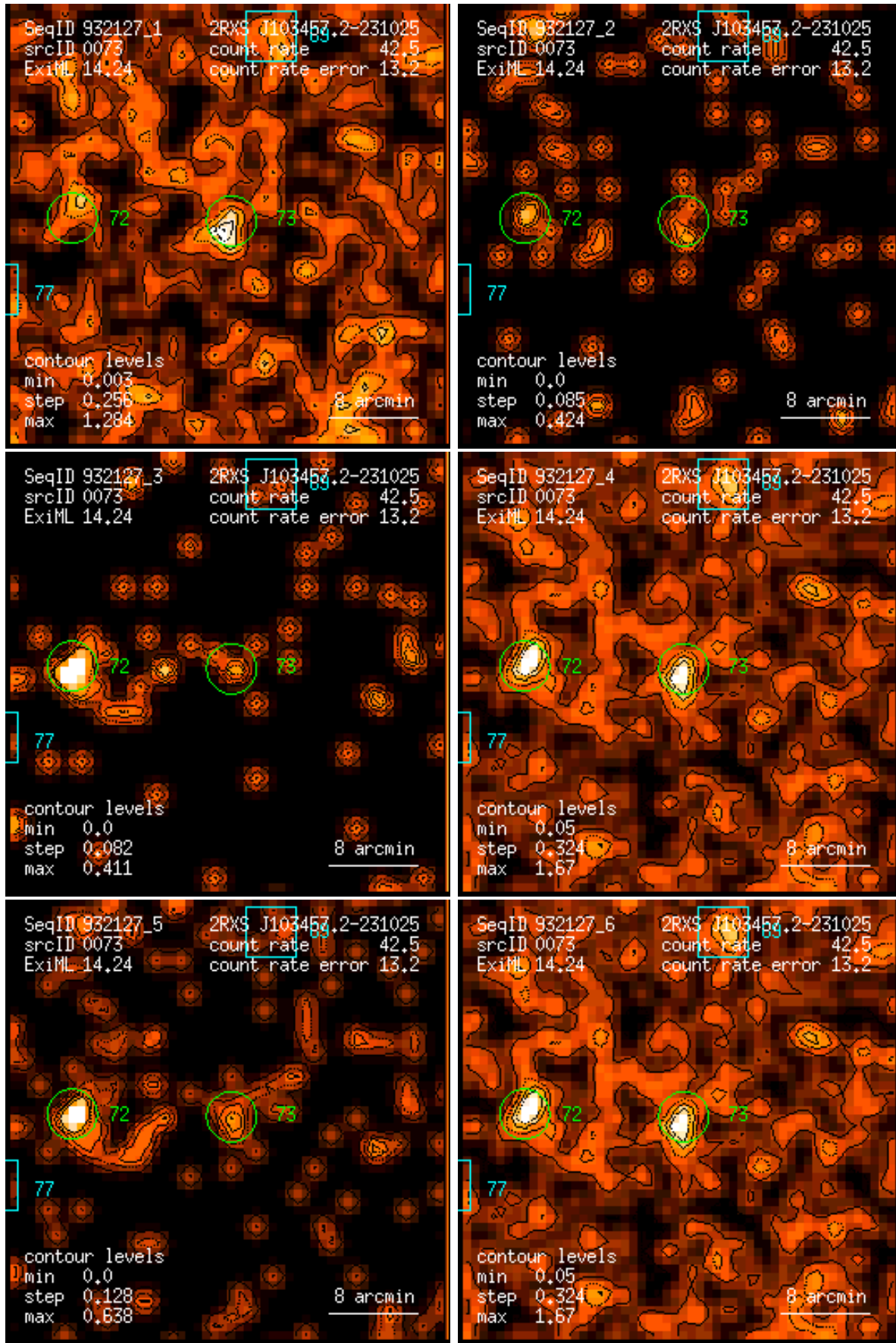
Figure 73: RASS 932127: detection 0073: band rate images, Gaussian filter: (1) PSPC channels 11 – 41, (2) 52 – 90, (3) 91 – 201, (4) 11 – 235, (5) 52 – 201, (6) 11 – 201. Broad band rates in counts/ks. Band rate contour levels in counts/ks/arcmin 2 .
