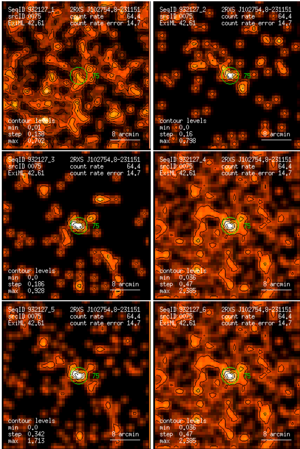
Figure 75: RASS 932127: detection 0075: band rate images, Gaussian filter: (1) PSPC channels 11 – 41, (2) 52 – 90, (3) 91 – 201, (4) 11 – 235, (5) 52 – 201, (6) 11 – 201. Broad band rates in counts/ks. Band rate contour levels in counts/ks/arcmin 2 .
