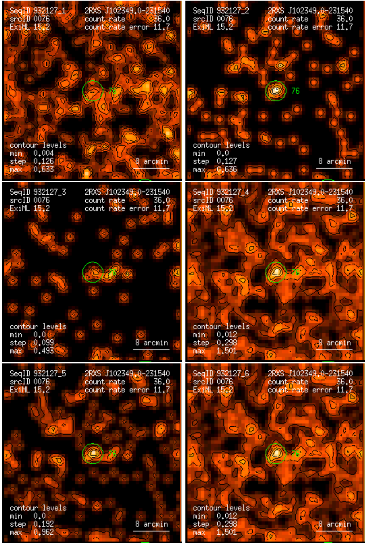
Figure 76: RASS 932127: detection 0076: band rate images, Gaussian filter: (1) PSPC channels 11 – 41, (2) 52 – 90, (3) 91 – 201, (4) 11 – 235, (5) 52 – 201, (6) 11 – 201. Broad band rates in counts/ks. Band rate contour levels in counts/ks/arcmin 2 .
