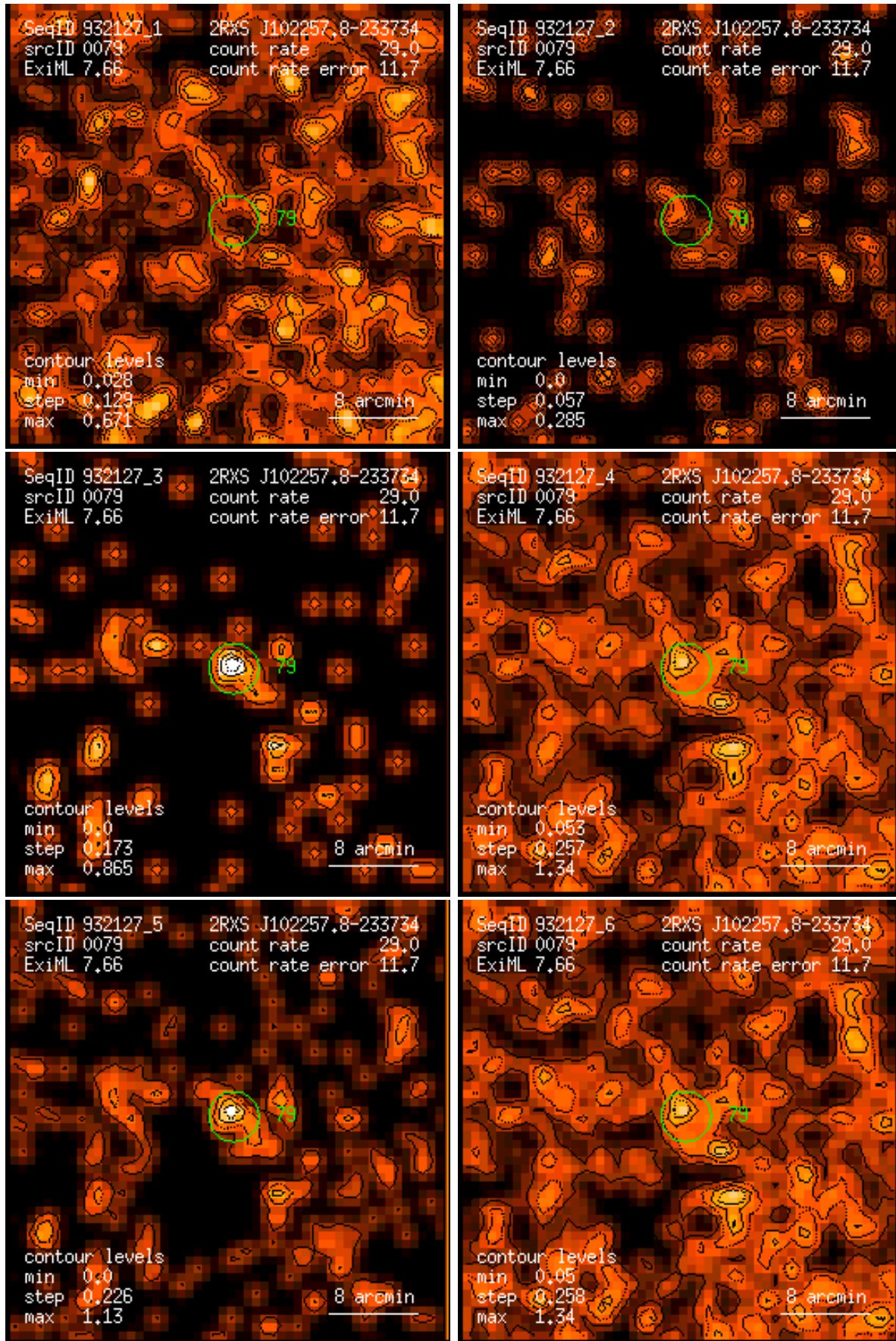
Figure 79: RASS 932127: detection 0079: band rate images, Gaussian filter: (1) PSPC channels 11 – 41, (2) 52 – 90, (3) 91 – 201, (4) 11 – 235, (5) 52 – 201, (6) 11 – 201. Broad band rates in counts/ks. Band rate contour levels in counts/ks/arcmin 2 .
