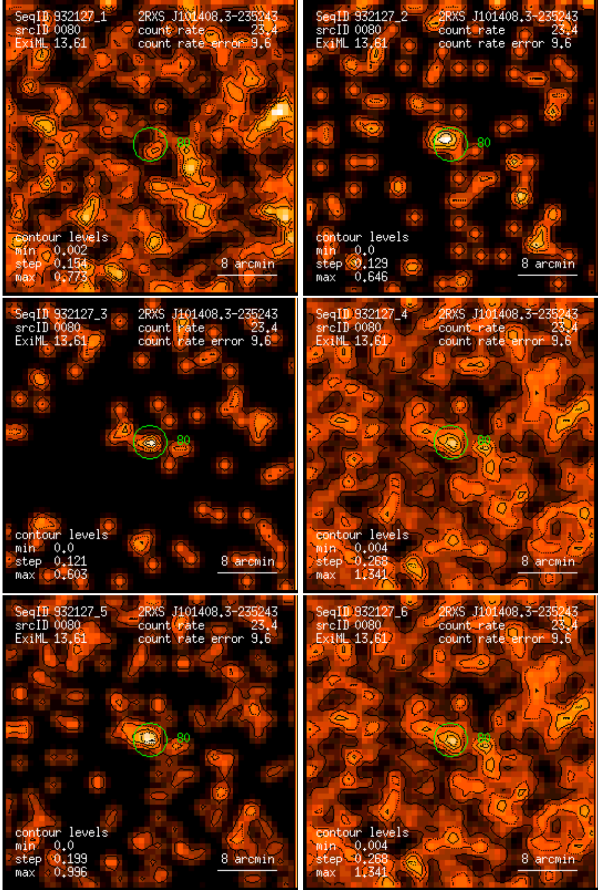
Figure 80: RASS 932127: detection 0080: band rate images, Gaussian filter: (1) PSPC channels 11 – 41, (2) 52 – 90, (3) 91 – 201, (4) 11 – 235, (5) 52 – 201, (6) 11 – 201. Broad band rates in counts/ks. Band rate contour levels in counts/ks/arcmin 2 .
