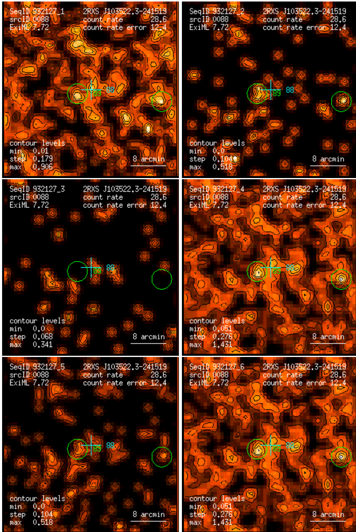
Figure 88: RASS 932127: detection 0088: band rate images, Gaussian filter: (1) PSPC channels 11 – 41, (2) 52 – 90, (3) 91 – 201, (4) 11 – 235, (5) 52 – 201, (6) 11 – 201. Broad band rates in counts/ks. Band rate contour levels in counts/ks/arcmin 2 .
