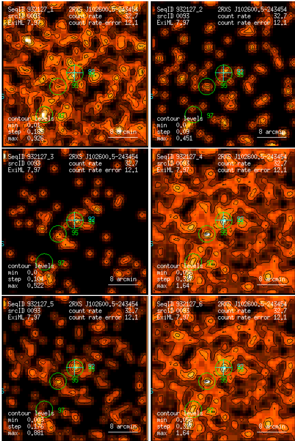
Figure 93: RASS 932127: detection 0093: band rate images, Gaussian filter: (1) PSPC channels 11 – 41, (2) 52 – 90, (3) 91 – 201, (4) 11 – 235, (5) 52 – 201, (6) 11 – 201. Broad band rates in counts/ks. Band rate contour levels in counts/ks/arcmin 2 .
