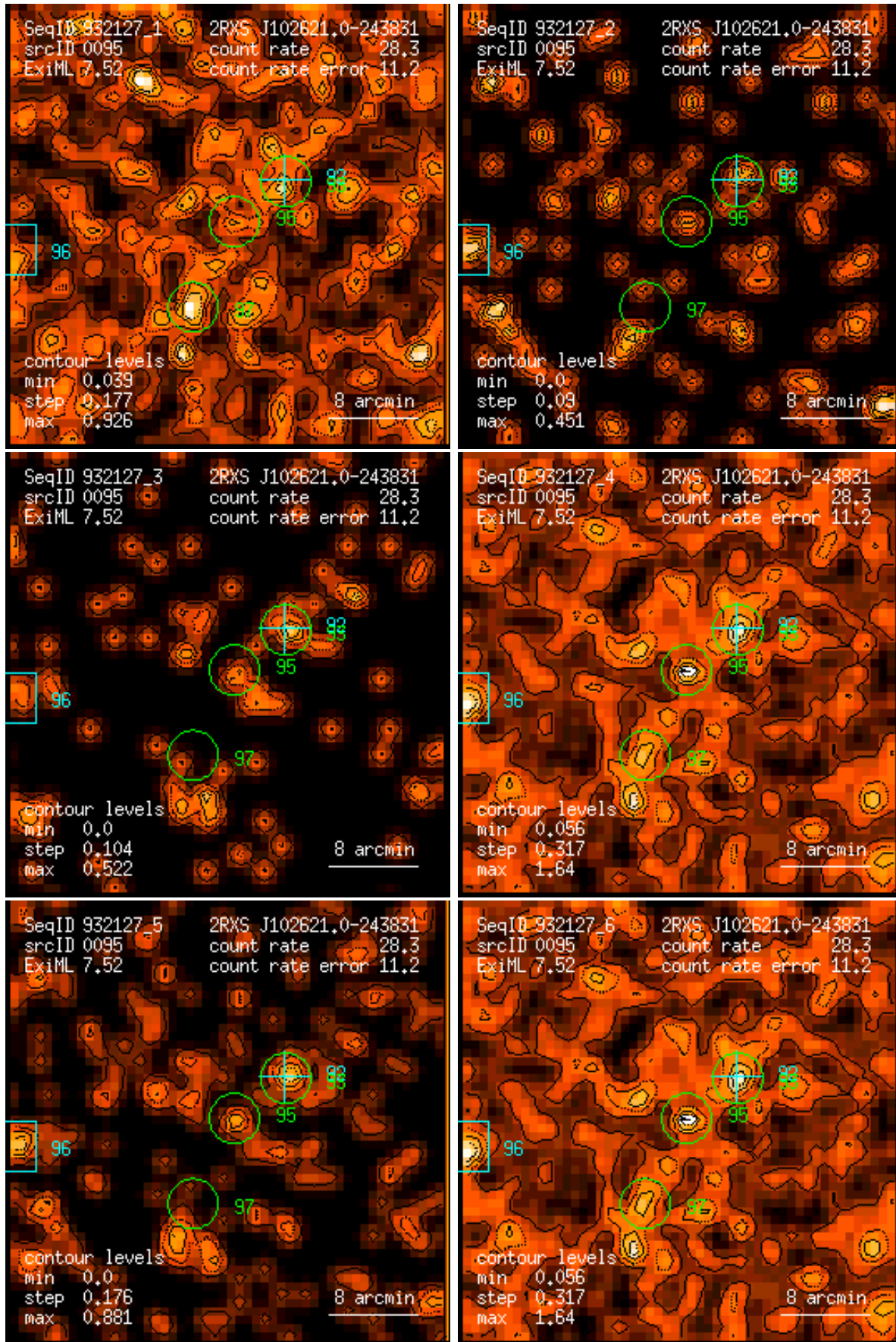
Figure 95: RASS 932127: detection 0095: band rate images, Gaussian filter: (1) PSPC channels 11 – 41, (2) 52 – 90, (3) 91 – 201, (4) 11 – 235, (5) 52 – 201, (6) 11 – 201. Broad band rates in counts/ks. Band rate contour levels in counts/ks/arcmin 2 .
